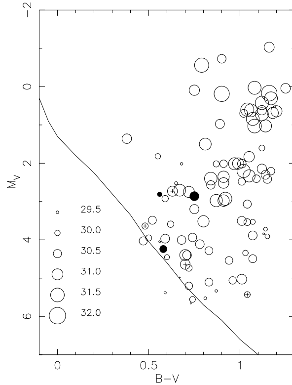
Fig. 4. X-ray luminosities of RS CVn systems detected in the ROSAT All Sky Survey (open circles; data from Dempsey et al. 1993) and detected in M 67 (filled circles), as a function of their location in the Hertzsprung Russell diagram. Colours and magnitudes are for the total light of the binary. The size of the symbols is proportional to the logarithm of the X-ray luminosity (in erg/s). The solid line indicates the main sequence. Four binaries in M 67 with unknown binary parameters presumably also are RS CVn systems, and are also shown (circles with inscribed +). Corrections for interstellar absorption have been made for the M 67 systems only; the corrections for the field systems are expected to be small. The X-ray luminosities for the RS CVn systems in M 67 are similar to those of the field systems.
