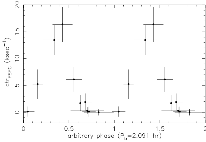
Fig. 2. The folded X-ray lightcurve of EU Cnc. The 100% variation is characteristic for AM-Her type systems.
