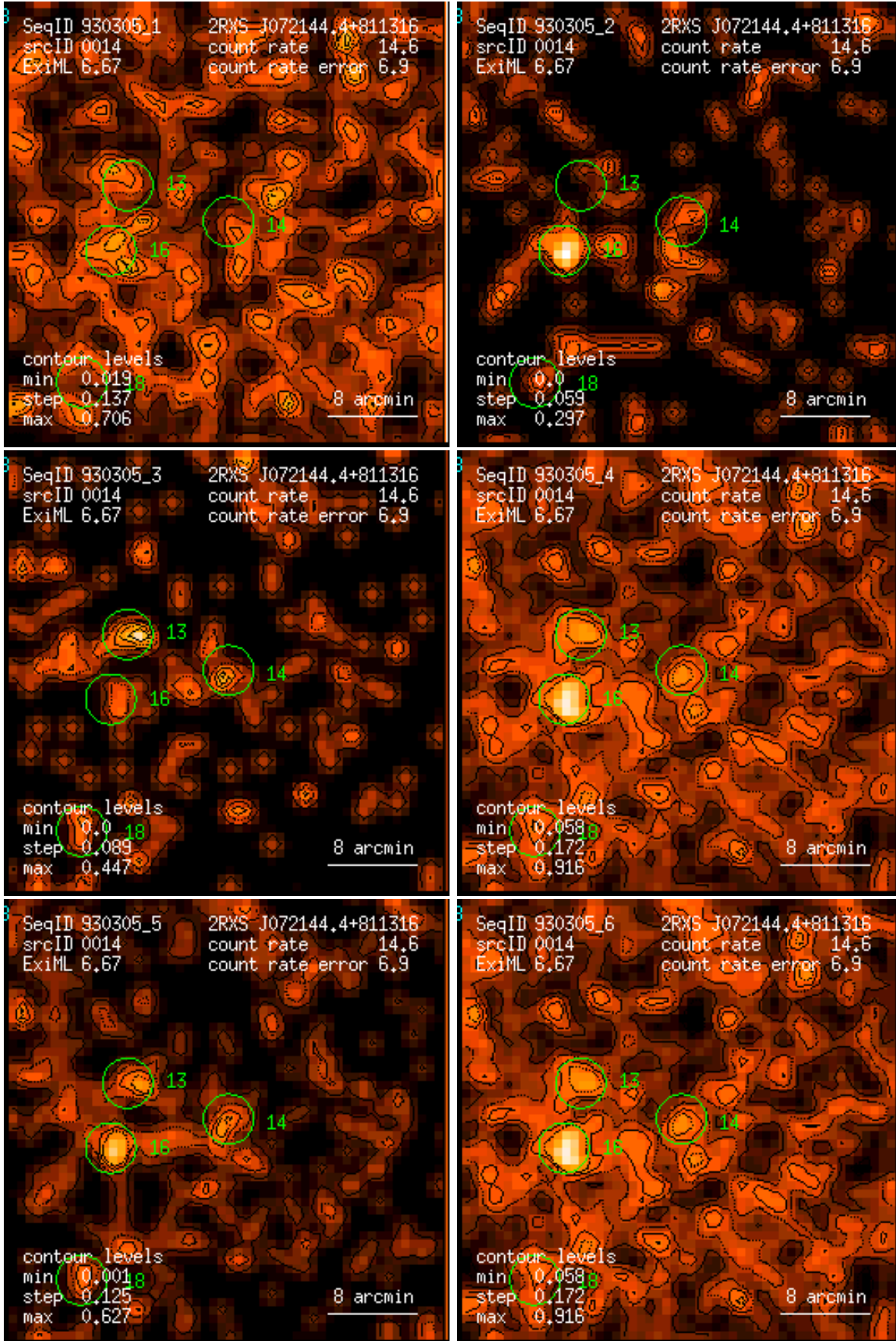
Figure 14: RASS 930305: detection 0014: band rate images, Gaussian filter: (1) PSPC channels 11 – 41, (2) 52 – 90, (3) 91 – 201, (4) 11 – 235, (5) 52 – 201, (6) 11 – 201. Broad band rates in counts/ks. Band rate contour levels in counts/ks/arcmin 2 .
