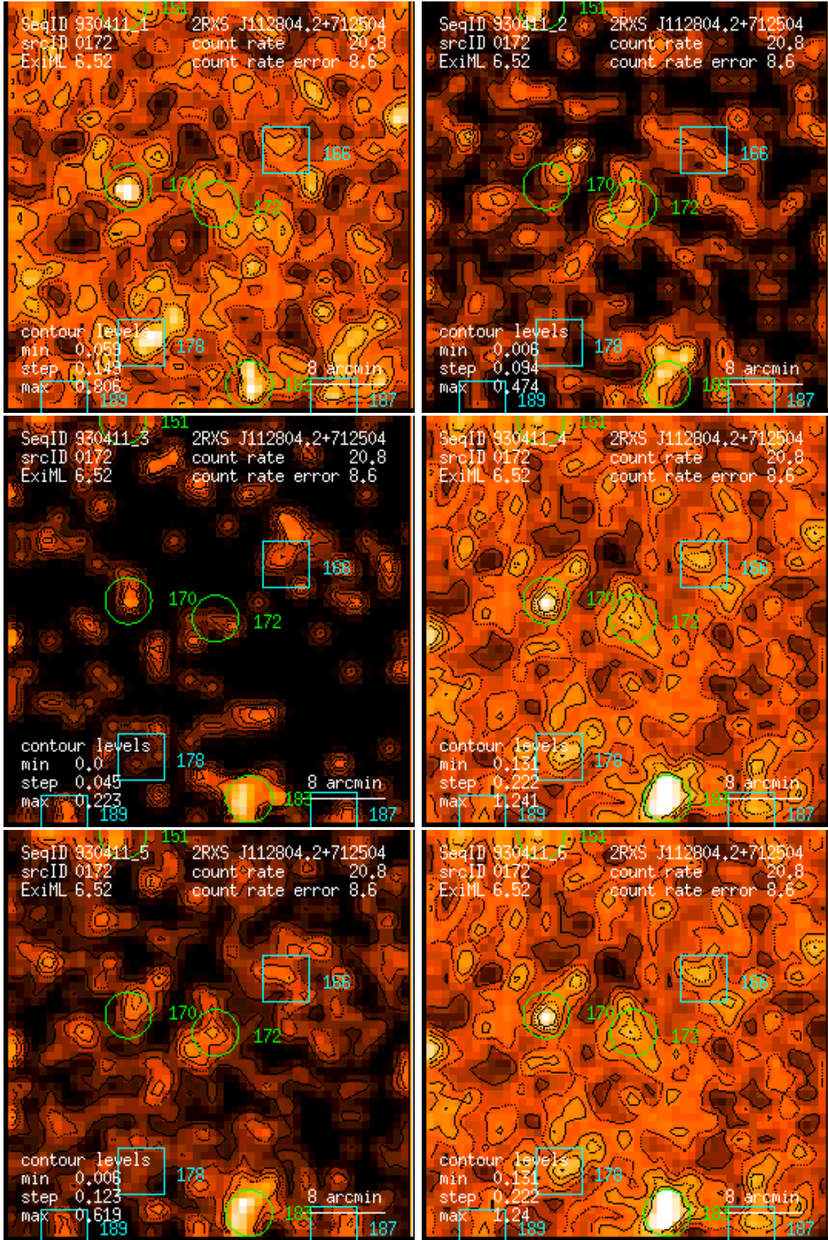
Figure 172: RASS 930411: detection 0172: band rate images, Gaussian filter: (1) PSPC channels 11 – 41, (2) 52 – 90, (3) 91 – 201, (4) 11 – 235, (5) 52 – 201, (6) 11 – 201. Broad band rates in counts/ks. Band rate contour levels in counts/ks/arcmin 2 .
