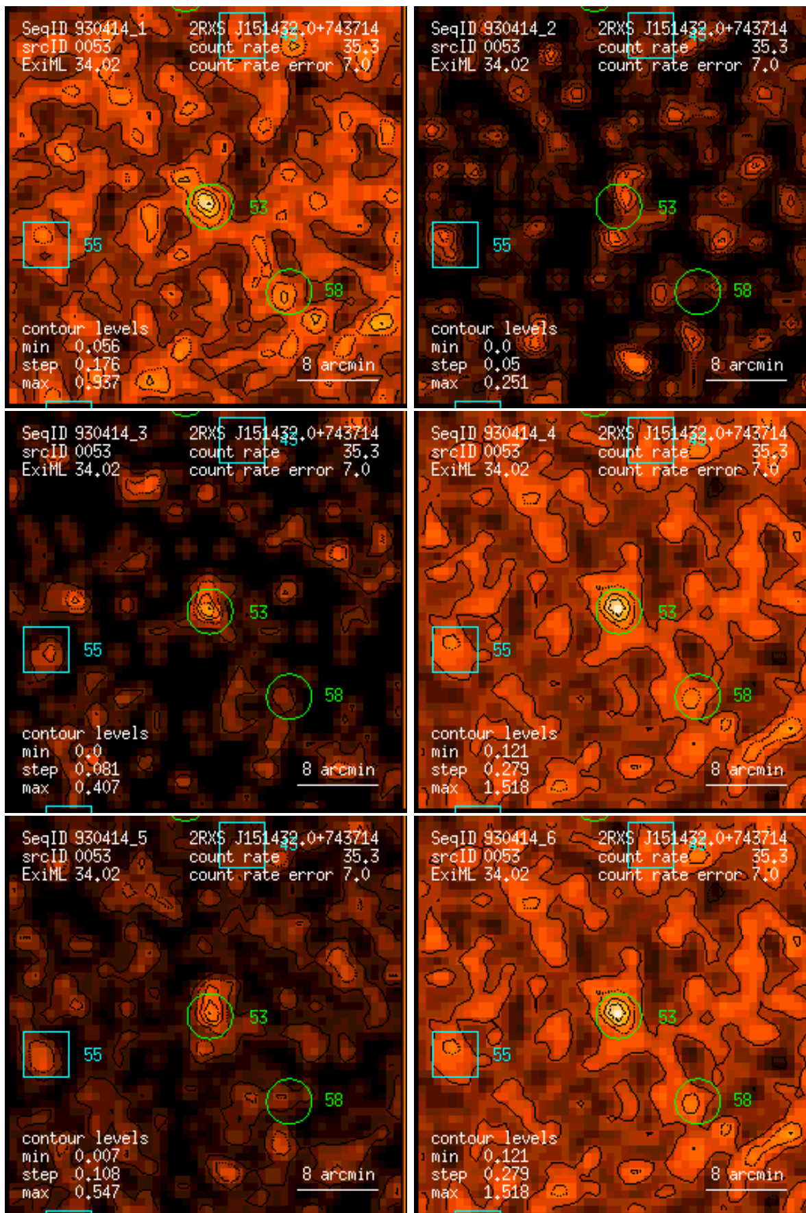
Figure 53: RASS 930414: detection 0053: band rate images, Gaussian filter: (1) PSPC channels 11 – 41, (2) 52 – 90, (3) 91 – 201, (4) 11 – 235, (5) 52 – 201, (6) 11 – 201. Broad band rates in counts/ks. Band rate contour levels in counts/ks/arcmin 2 .
