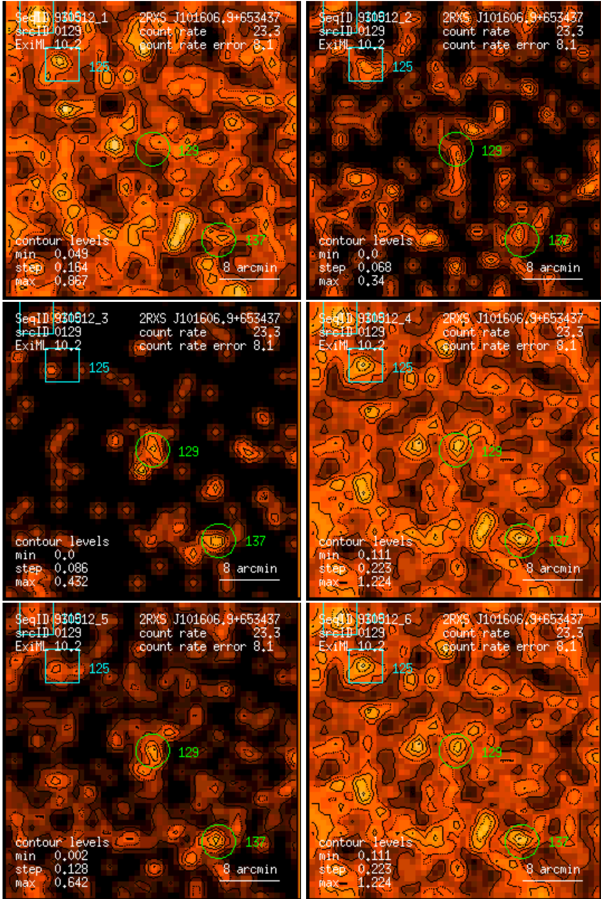
Figure 129: RASS 930512: detection 0129: band rate images, Gaussian filter: (1) PSPC channels 11 – 41, (2) 52 – 90, (3) 91 – 201, (4) 11 – 235, (5) 52 – 201, (6) 11 – 201. Broad band rates in counts/ks. Band rate contour levels in counts/ks/arcmin 2 .
