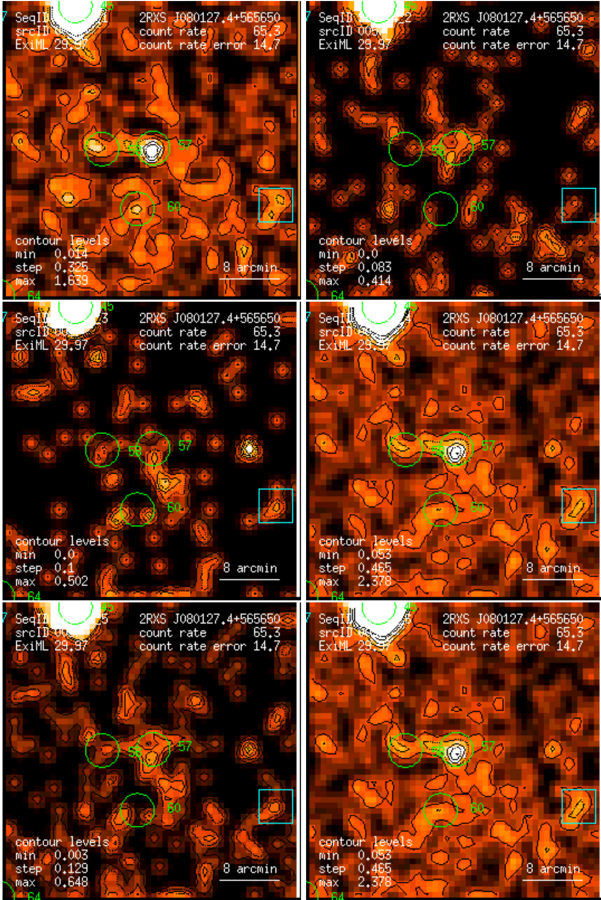
Figure 57: RASS 930714: detection 0057: band rate images, Gaussian filter: (1) PSPC channels 11 – 41, (2) 52 – 90, (3) 91 – 201, (4) 11 – 235, (5) 52 – 201, (6) 11 – 201. Broad band rates in counts/ks. Band rate contour levels in counts/ks/arcmin 2 .
