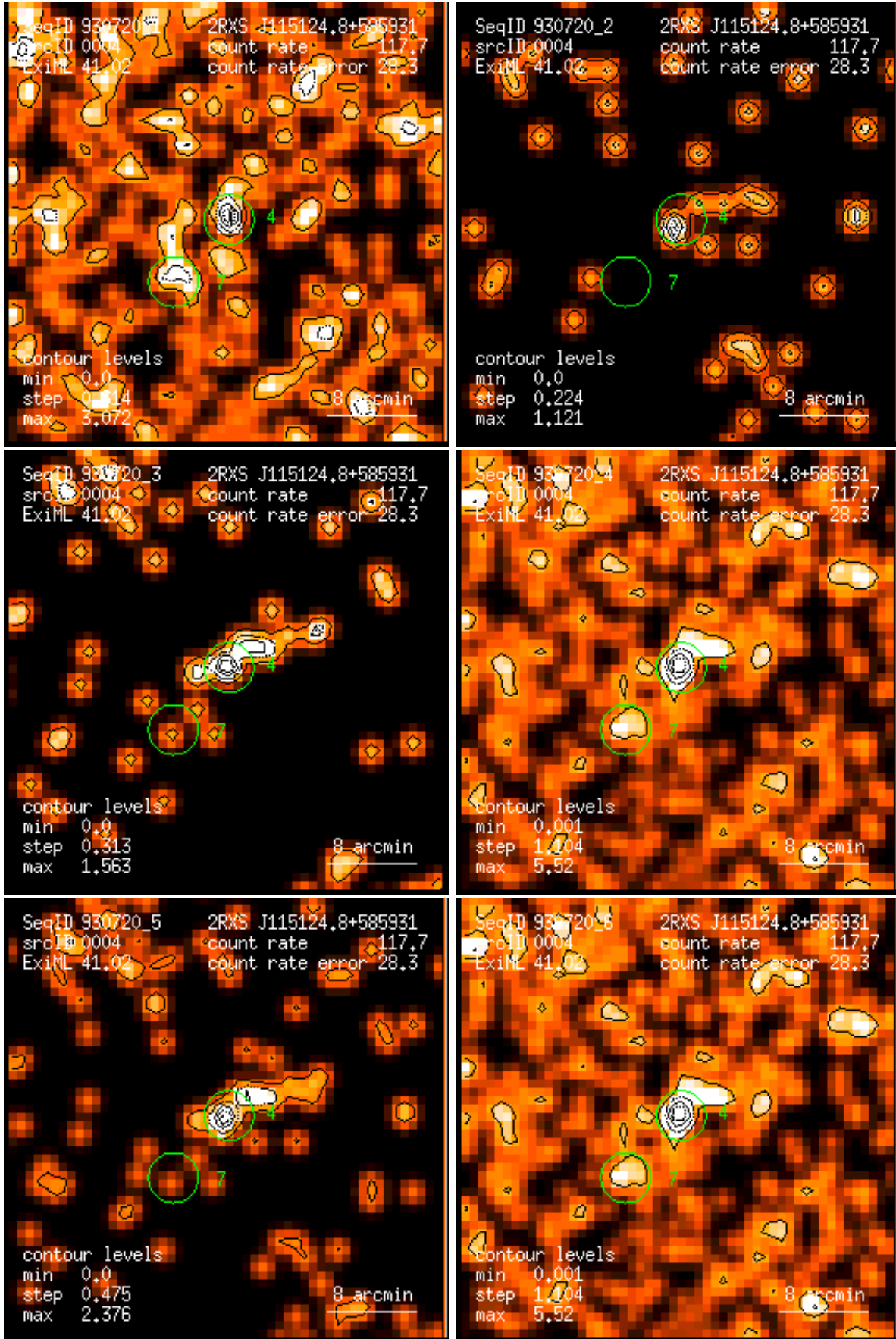
Figure 4: RASS 930720: detection 0004: band rate images, Gaussian filter: (1) PSPC channels 11 – 41, (2) 52 – 90, (3) 91 – 201, (4) 11 – 235, (5) 52 – 201, (6) 11 – 201. Broad band rates in counts/ks. Band rate contour levels in counts/ks/arcmin 2 .
