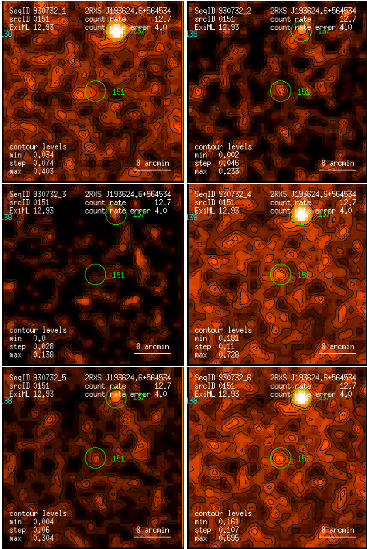
Figure 151: RASS 930732: detection 0151: band rate images, Gaussian filter: (1) PSPC channels 11 – 41, (2) 52 – 90, (3) 91 – 201, (4) 11 – 235, (5) 52 – 201, (6) 11 – 201. Broad band rates in counts/ks. Band rate contour levels in counts/ks/arcmin 2 .
