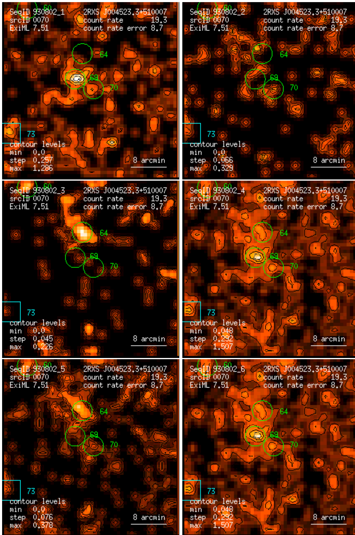
Figure 70: RASS 930802: detection 0070: band rate images, Gaussian filter: (1) PSPC channels 11 – 41, (2) 52 – 90, (3) 91 – 201, (4) 11 – 235, (5) 52 – 201, (6) 11 – 201. Broad band rates in counts/ks. Band rate contour levels in counts/ks/arcmin 2 .
