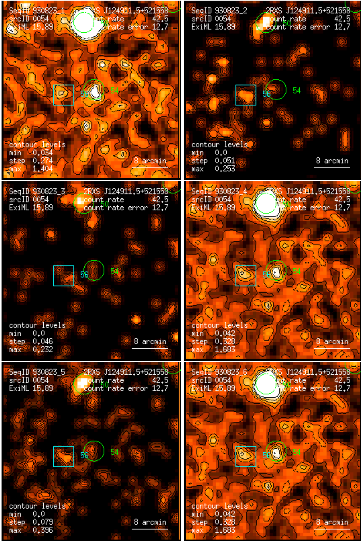
Figure 54: RASS 930823: detection 0054: band rate images, Gaussian filter: (1) PSPC channels 11 – 41, (2) 52 – 90, (3) 91 – 201, (4) 11 – 235, (5) 52 – 201, (6) 11 – 201. Broad band rates in counts/ks. Band rate contour levels in counts/ks/arcmin 2 .
