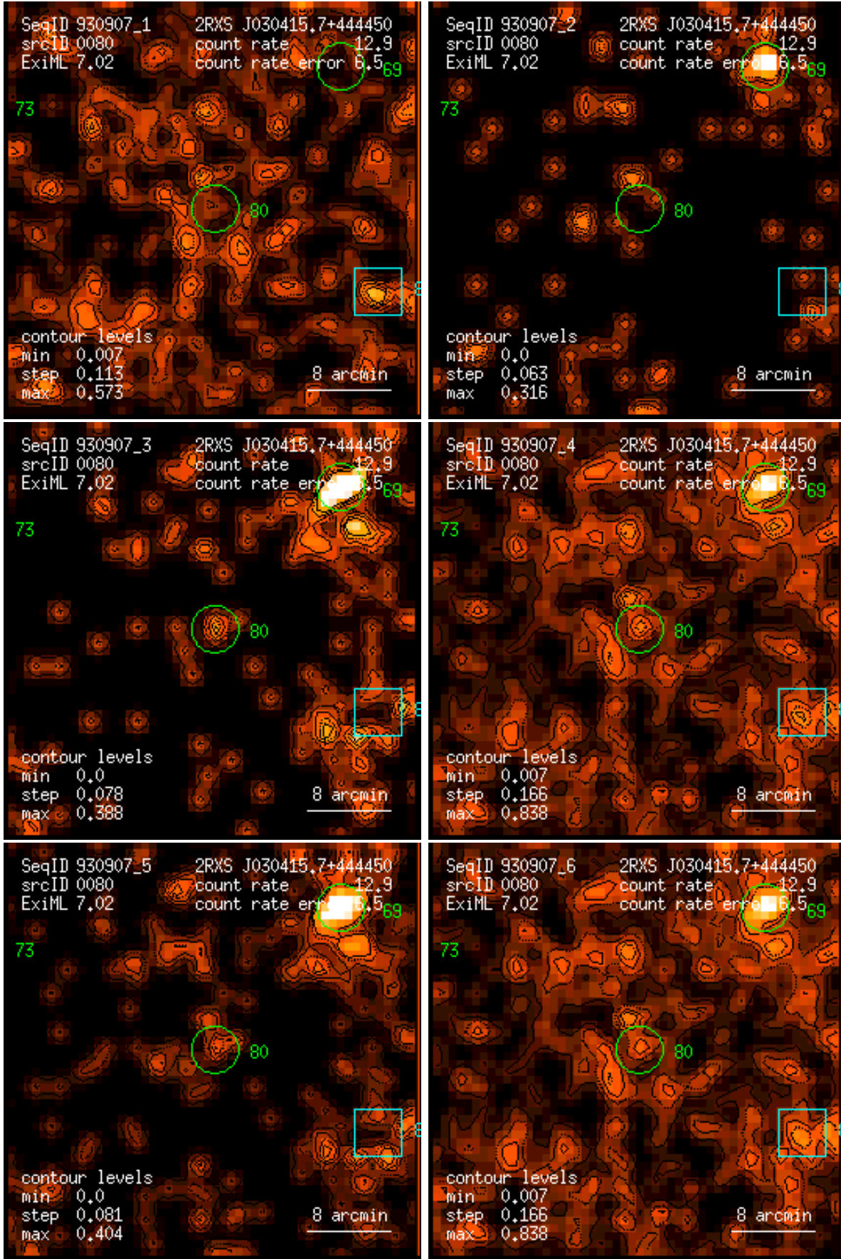
Figure 80: RASS 930907: detection 0080: band rate images, Gaussian filter: (1) PSPC channels 11 – 41, (2) 52 – 90, (3) 91 – 201, (4) 11 – 235, (5) 52 – 201, (6) 11 – 201. Broad band rates in counts/ks. Band rate contour levels in counts/ks/arcmin 2 .
