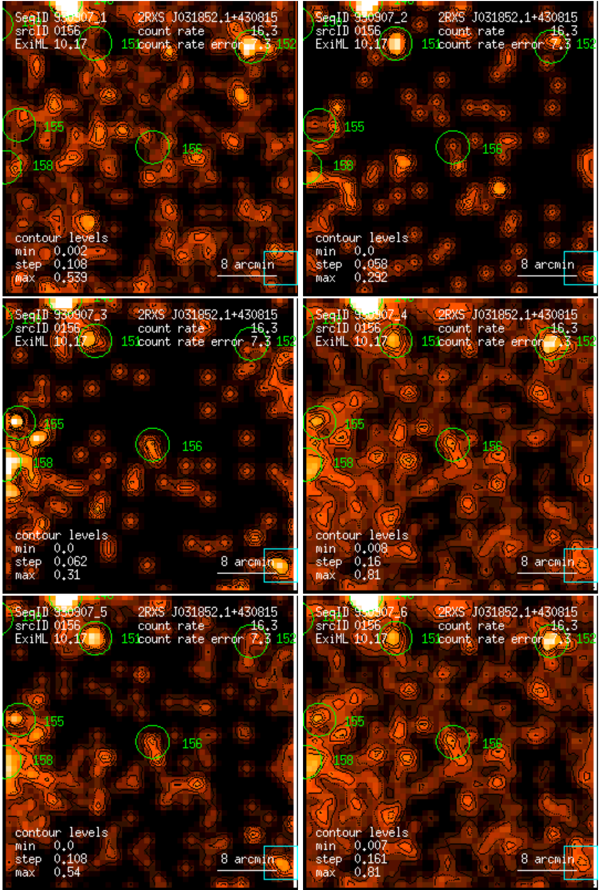
Figure 156: RASS 930907: detection 0156: band rate images, Gaussian filter: (1) PSPC channels 11 – 41, (2) 52 – 90, (3) 91 – 201, (4) 11 – 235, (5) 52 – 201, (6) 11 – 201. Broad band rates in counts/ks. Band rate contour levels in counts/ks/arcmin 2 .
