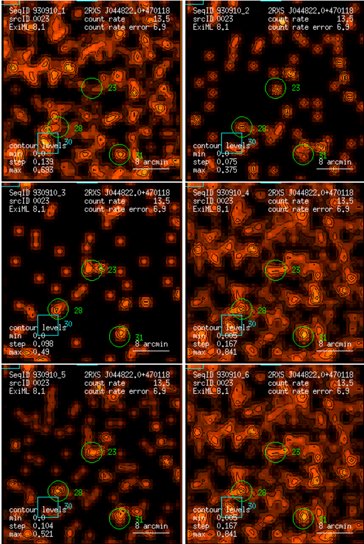
Figure 23: RASS 930910: detection 0023: band rate images, Gaussian filter: (1) PSPC channels 11 – 41, (2) 52 – 90, (3) 91 – 201, (4) 11 – 235, (5) 52 – 201, (6) 11 – 201. Broad band rates in counts/ks. Band rate contour levels in counts/ks/arcmin 2 .
