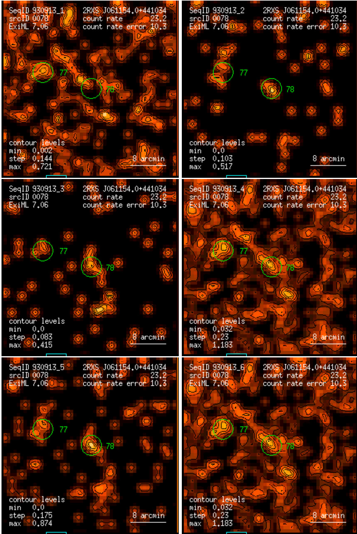
Figure 78: RASS 930913: detection 0078: band rate images, Gaussian filter: (1) PSPC channels 11 – 41, (2) 52 – 90, (3) 91 – 201, (4) 11 – 235, (5) 52 – 201, (6) 11 – 201. Broad band rates in counts/ks. Band rate contour levels in counts/ks/arcmin 2 .
