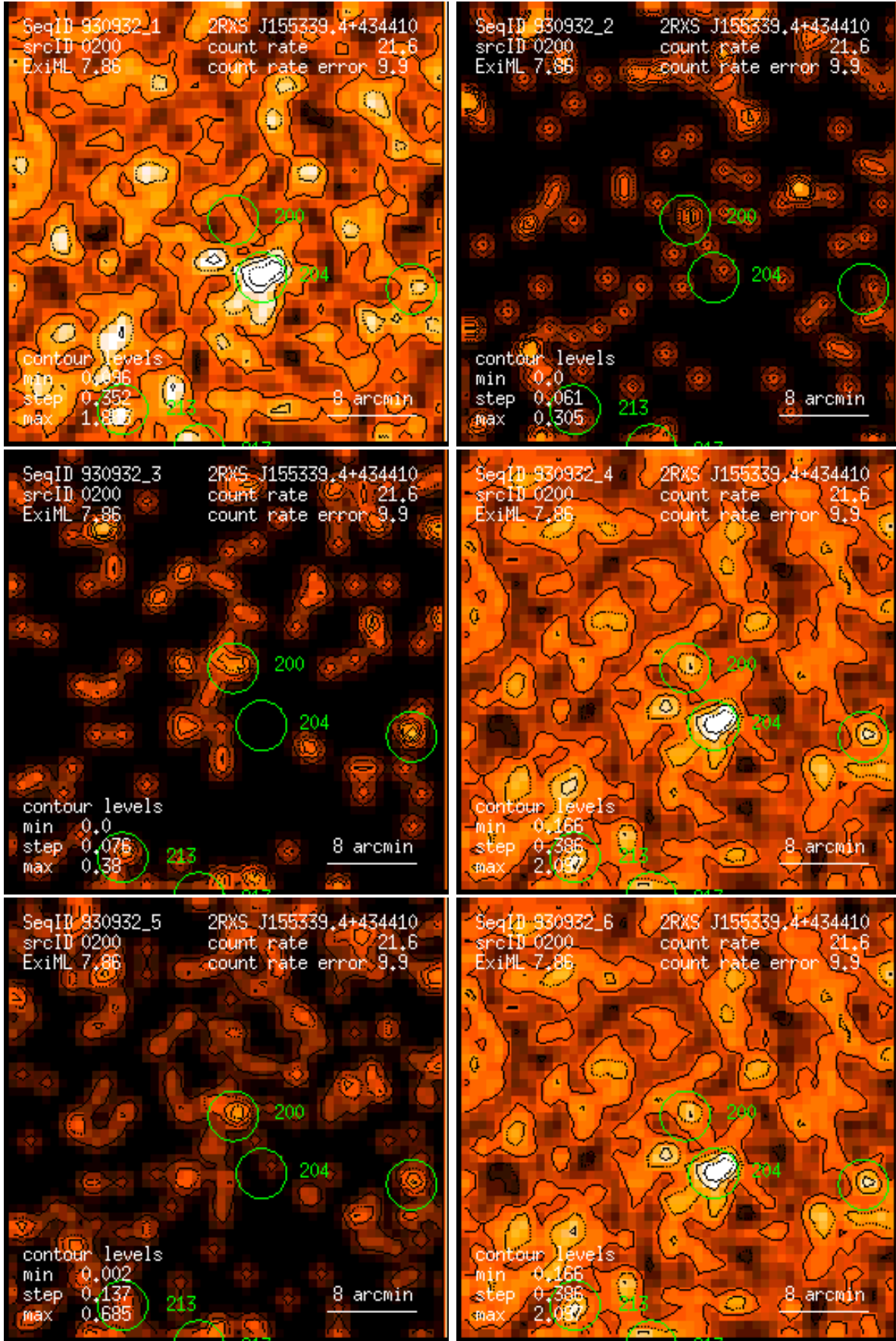
Figure 200: RASS 930932: detection 0200: band rate images, Gaussian filter: (1) PSPC channels 11 – 41, (2) 52 – 90, (3) 91 – 201, (4) 11 – 235, (5) 52 – 201, (6) 11 – 201. Broad band rates in counts/ks. Band rate contour levels in counts/ks/arcmin 2 .
