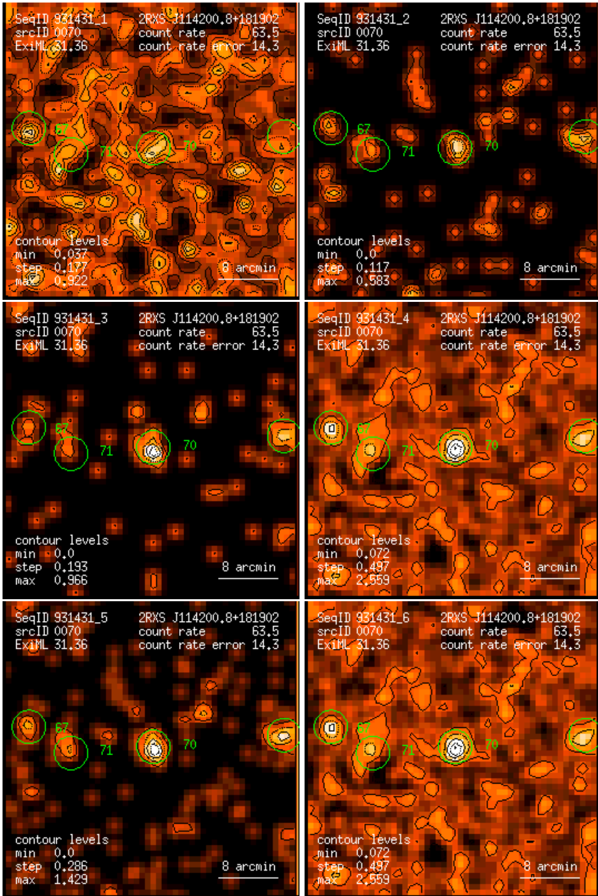
Figure 70: RASS 931431: detection 0070: band rate images, Gaussian filter: (1) PSPC channels 11 – 41, (2) 52 – 90, (3) 91 – 201, (4) 11 – 235, (5) 52 – 201, (6) 11 – 201. Broad band rates in counts/ks. Band rate contour levels in counts/ks/arcmin 2 .
