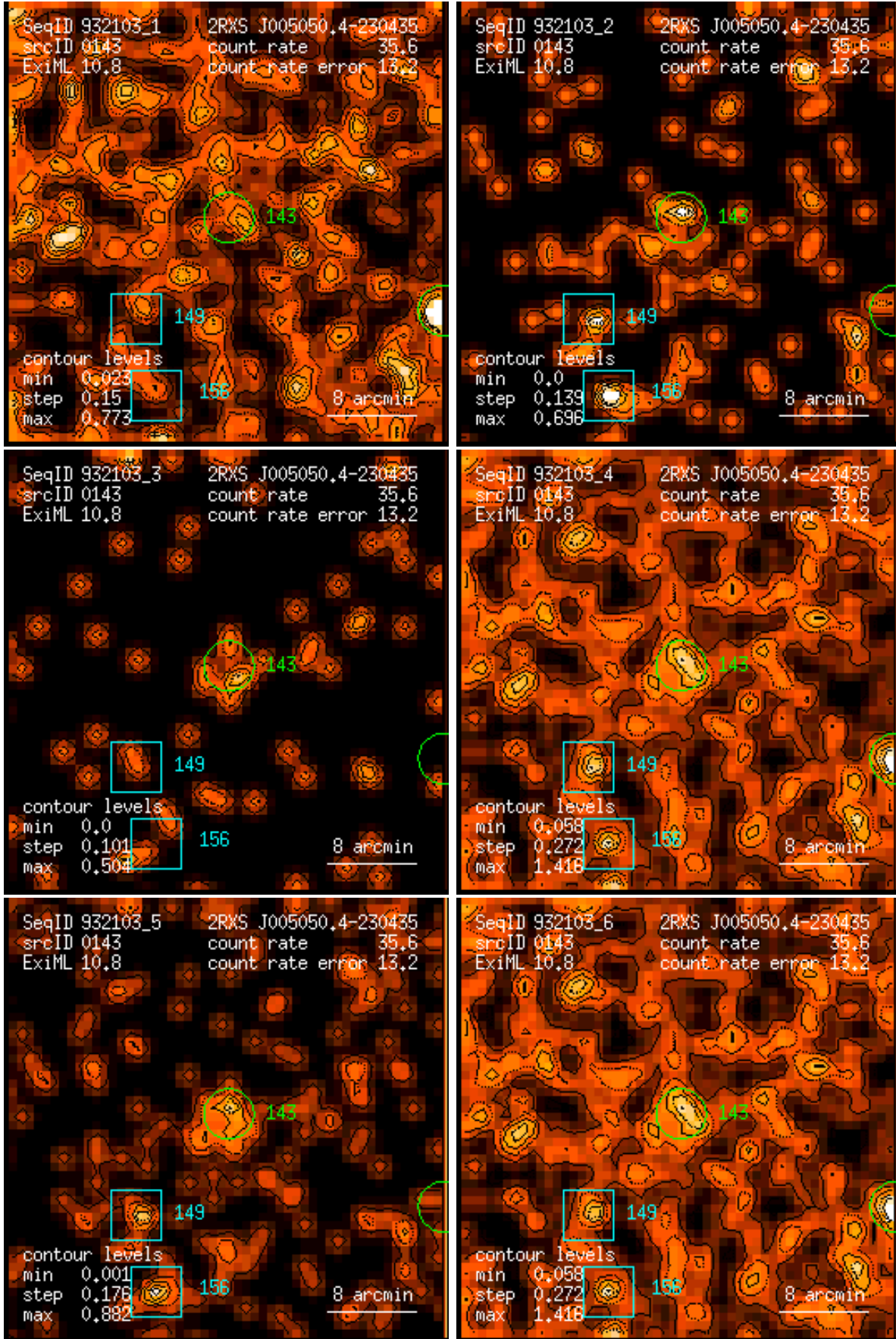
Figure 143: RASS 932103: detection 0143: band rate images, Gaussian filter: (1) PSPC channels 11 – 41, (2) 52 – 90, (3) 91 – 201, (4) 11 – 235, (5) 52 – 201, (6) 11 – 201. Broad band rates in counts/ks. Band rate contour levels in counts/ks/arcmin 2 .
