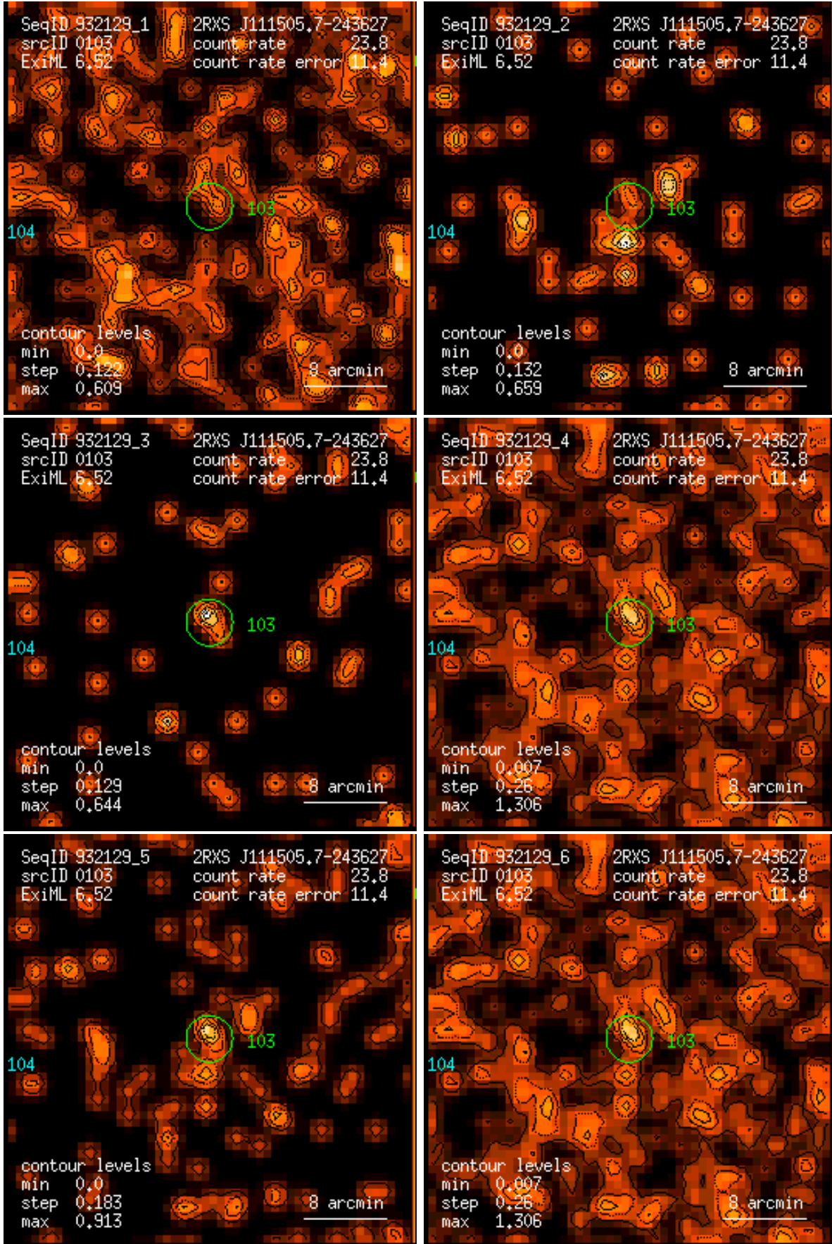
Figure 103: RASS 932129: detection 0103: band rate images, Gaussian filter: (1) PSPC channels 11 – 41, (2) 52 – 90, (3) 91 – 201, (4) 11 – 235, (5) 52 – 201, (6) 11 – 201. Broad band rates in counts/ks. Band rate contour levels in counts/ks/arcmin 2 .
