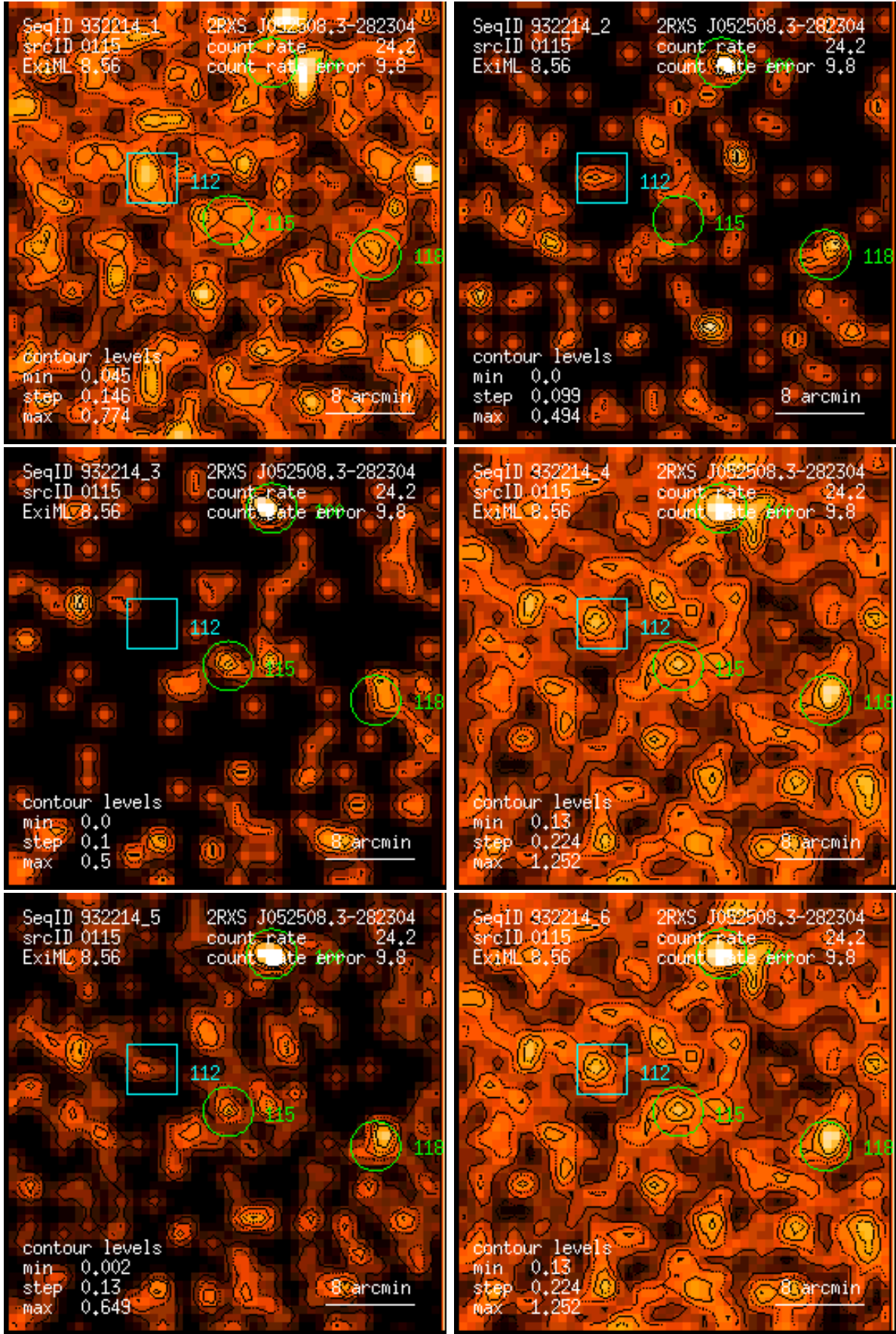
Figure 115: RASS 932214: detection 0115: band rate images, Gaussian filter: (1) PSPC channels 11 – 41, (2) 52 – 90, (3) 91 – 201, (4) 11 – 235, (5) 52 – 201, (6) 11 – 201. Broad band rates in counts/ks. Band rate contour levels in counts/ks/arcmin 2 .
