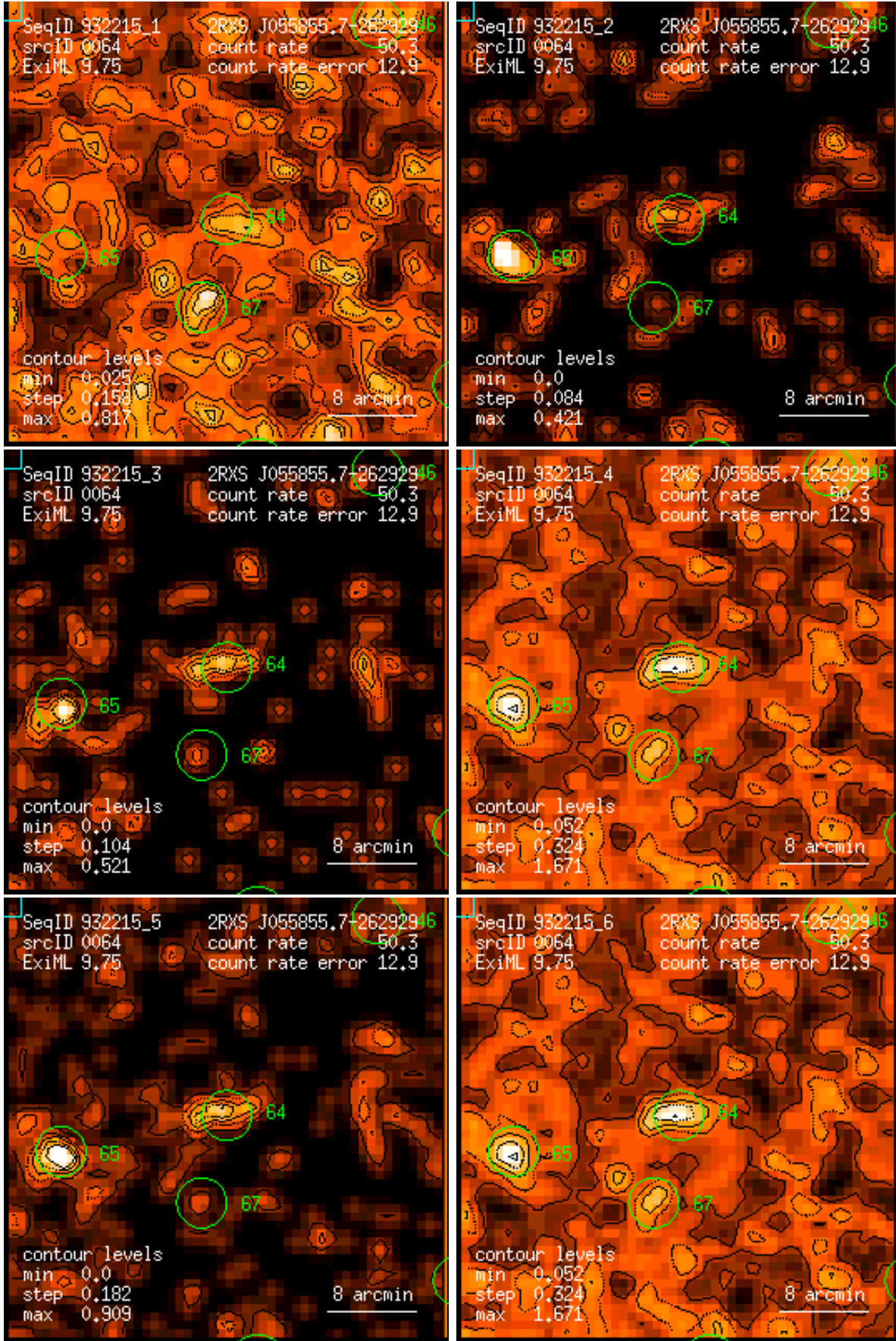
Figure 64: RASS 932215: detection 0064: band rate images, Gaussian filter: (1) PSPC channels 11 – 41, (2) 52 – 90, (3) 91 – 201, (4) 11 – 235, (5) 52 – 201, (6) 11 – 201. Broad band rates in counts/ks. Band rate contour levels in counts/ks/arcmin 2 .
