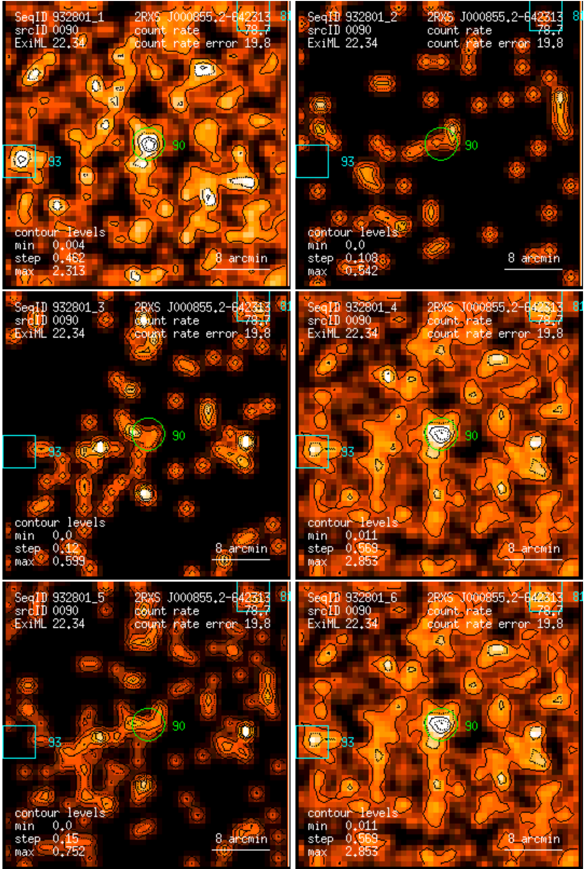
Figure 90: RASS 932801: detection 0090: band rate images, Gaussian filter: (1) PSPC channels 11 – 41, (2) 52 – 90, (3) 91 – 201, (4) 11 – 235, (5) 52 – 201, (6) 11 – 201. Broad band rates in counts/ks. Band rate contour levels in counts/ks/arcmin 2 .
