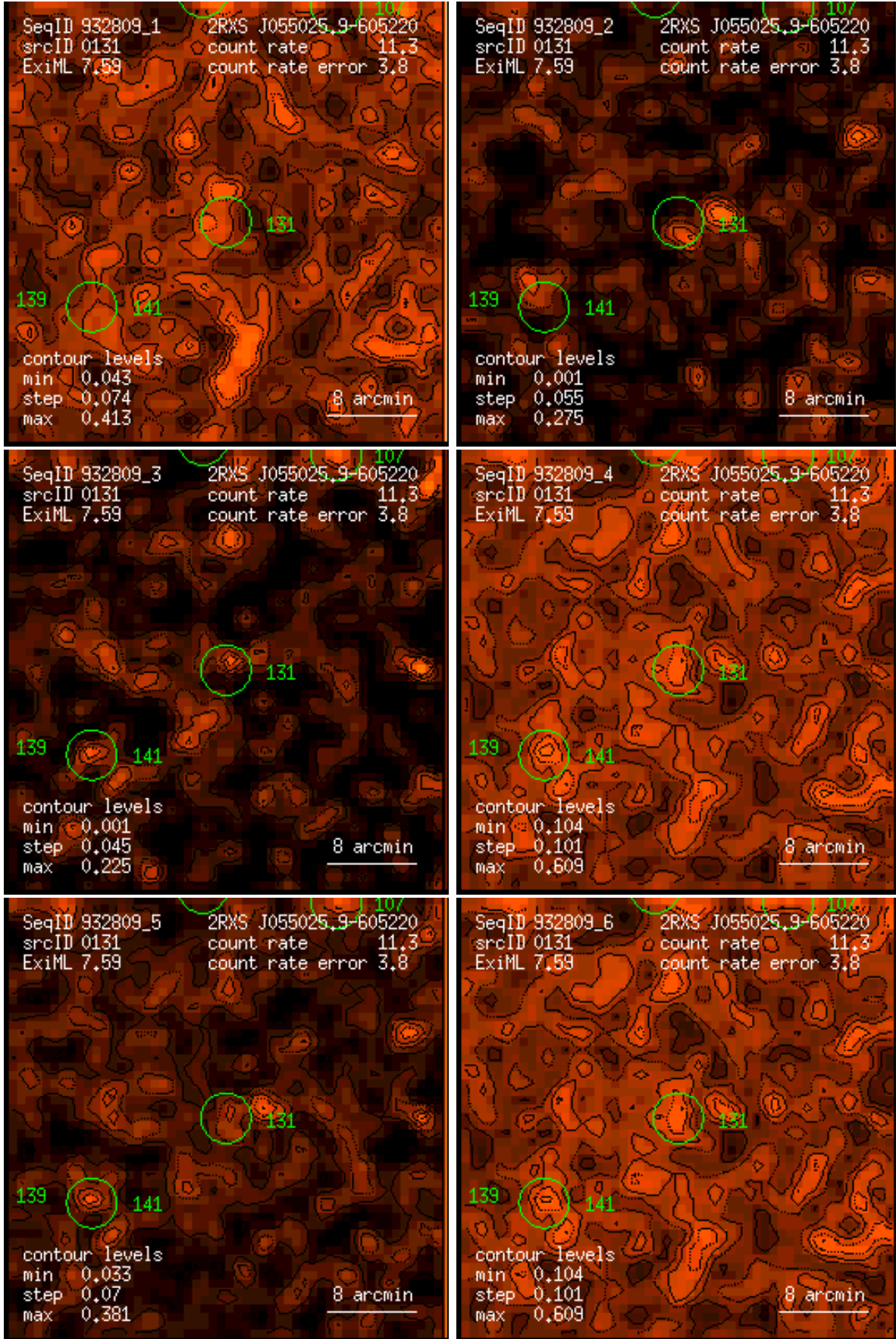
Figure 131: RASS 932809: detection 0131: band rate images, Gaussian filter: (1) PSPC channels 11 – 41, (2) 52 – 90, (3) 91 – 201, (4) 11 – 235, (5) 52 – 201, (6) 11 – 201. Broad band rates in counts/ks. Band rate contour levels in counts/ks/arcmin 2 .
