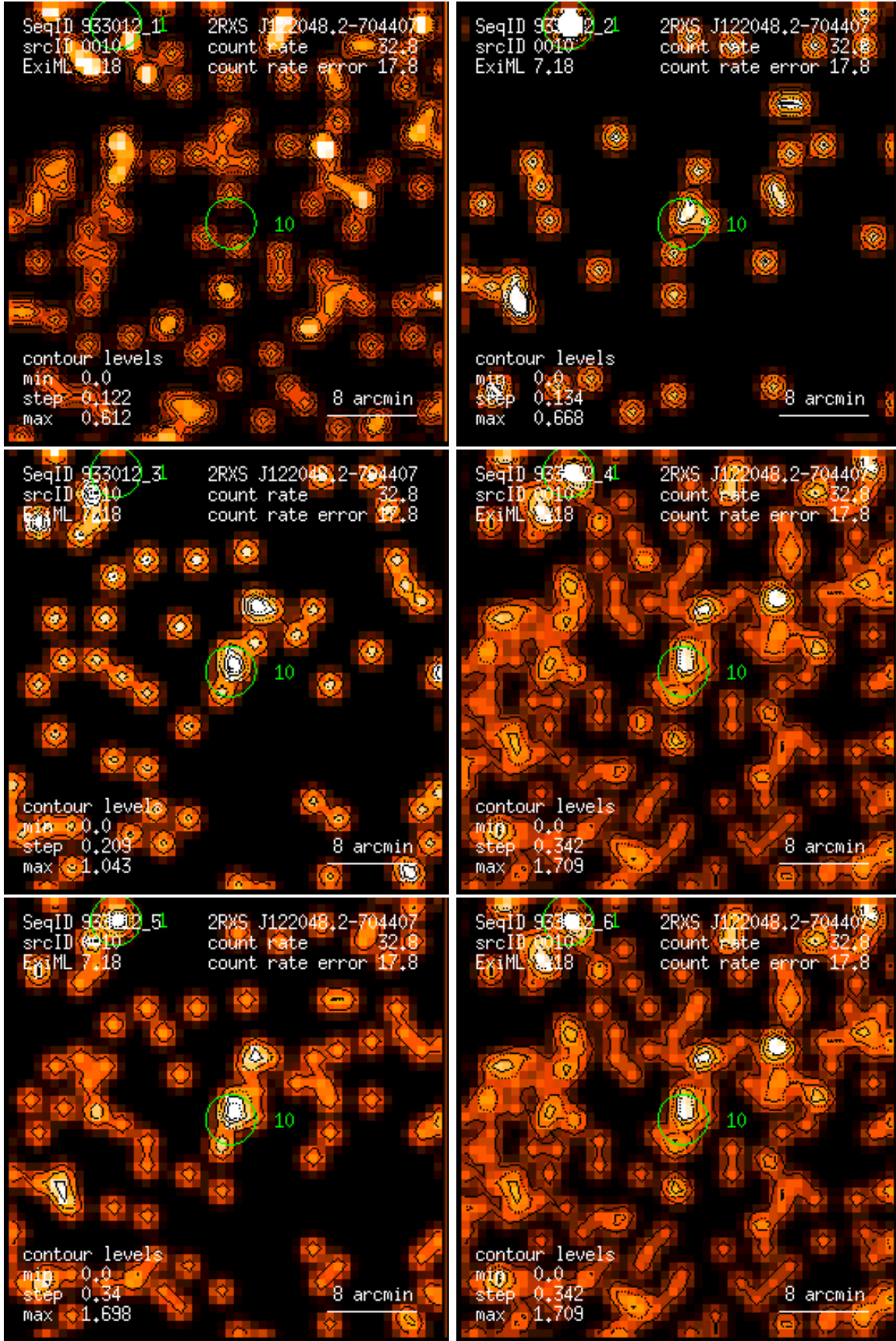
Figure 10: RASS 933012: detection 0010: band rate images, Gaussian filter: (1) PSPC channels 11 – 41, (2) 52 – 90, (3) 91 – 201, (4) 11 – 235, (5) 52 – 201, (6) 11 – 201. Broad band rates in counts/ks. Band rate contour levels in counts/ks/arcmin 2 .
