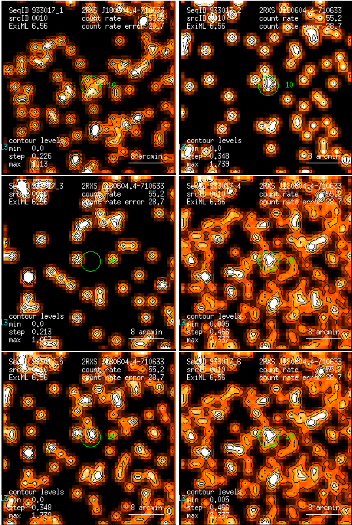
Figure 10: RASS 933017: detection 0010: band rate images, Gaussian filter: (1) PSPC channels 11 – 41, (2) 52 – 90, (3) 91 – 201, (4) 11 – 235, (5) 52 – 201, (6) 11 – 201. Broad band rates in counts/ks. Band rate contour levels in counts/ks/arcmin 2 .
