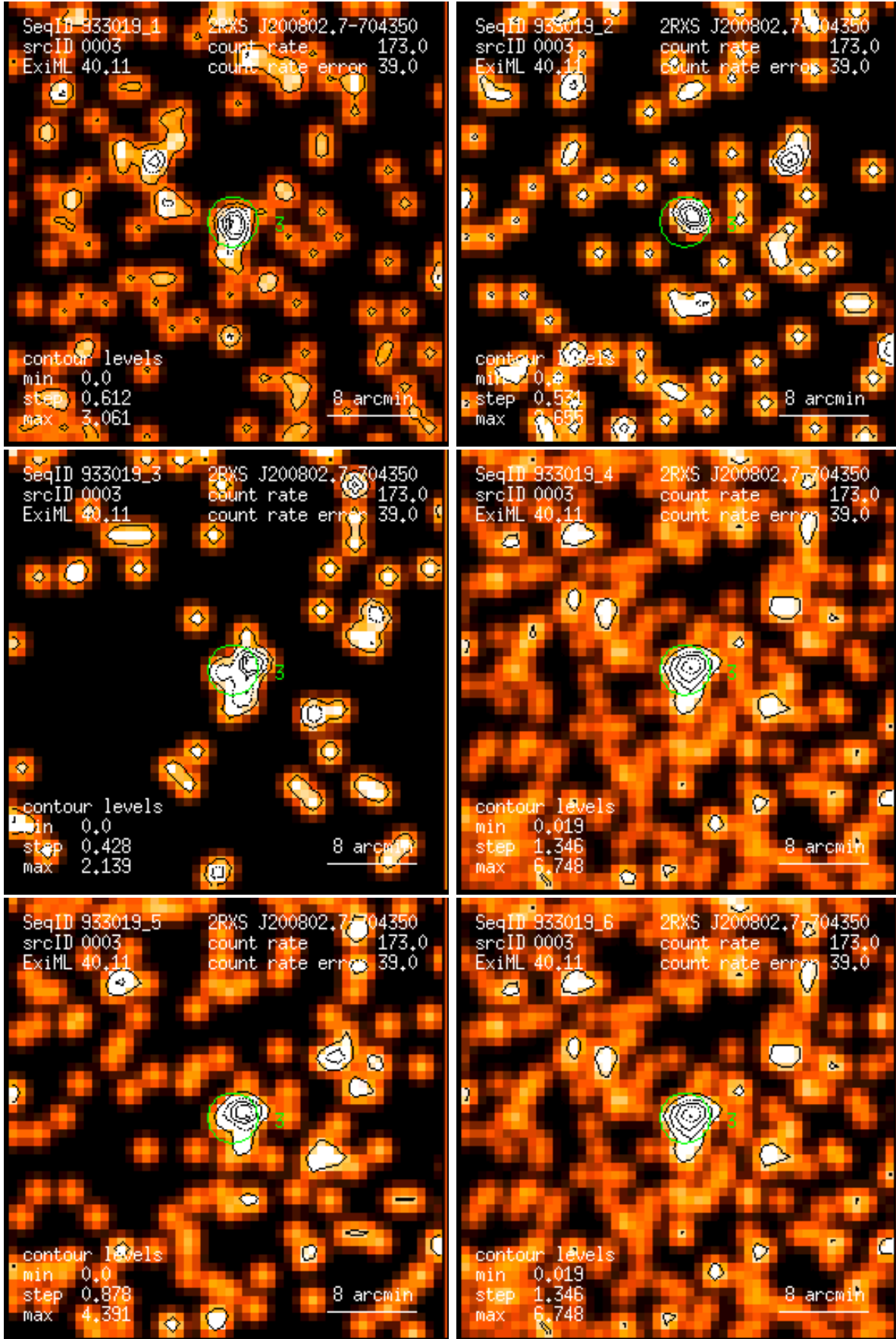
Figure 3: RASS 933019: detection 0003: band rate images, Gaussian filter: (1) PSPC channels 11 – 41, (2) 52 – 90, (3) 91 – 201, (4) 11 – 235, (5) 52 – 201, (6) 11 – 201. Broad band rates in counts/ks. Band rate contour levels in counts/ks/arcmin 2 .
