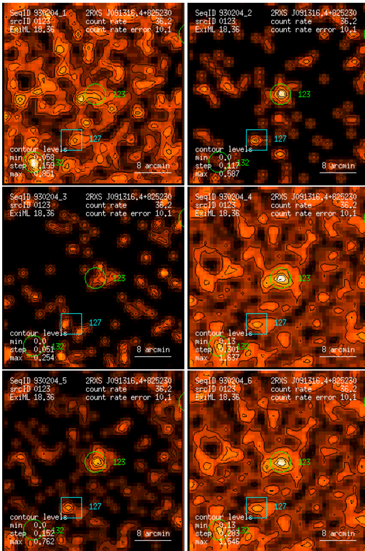
Figure 123: RASS 930204: detection 0123: band rate images, Gaussian filter: (1) PSPC channels 11 – 41, (2) 52 – 90, (3) 91 – 201, (4) 11 – 235, (5) 52 – 201, (6) 11 – 201. Broad band rates in counts/ks. Band rate contour levels in counts/ks/arcmin 2 .
