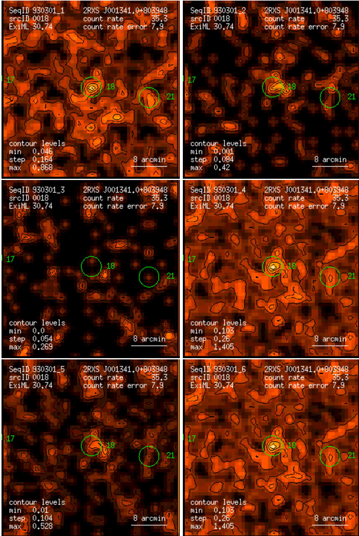
Figure 18: RASS 930301: detection 0018: band rate images, Gaussian filter: (1) PSPC channels 11 – 41, (2) 52 – 90, (3) 91 – 201, (4) 11 – 235, (5) 52 – 201, (6) 11 – 201. Broad band rates in counts/ks. Band rate contour levels in counts/ks/arcmin 2 .
