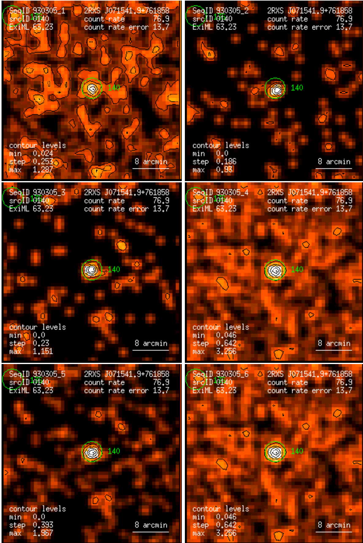
Figure 140: RASS 930305: detection 0140: band rate images, Gaussian filter: (1) PSPC channels 11 – 41, (2) 52 – 90, (3) 91 – 201, (4) 11 – 235, (5) 52 – 201, (6) 11 – 201. Broad band rates in counts/ks. Band rate contour levels in counts/ks/arcmin 2 .
