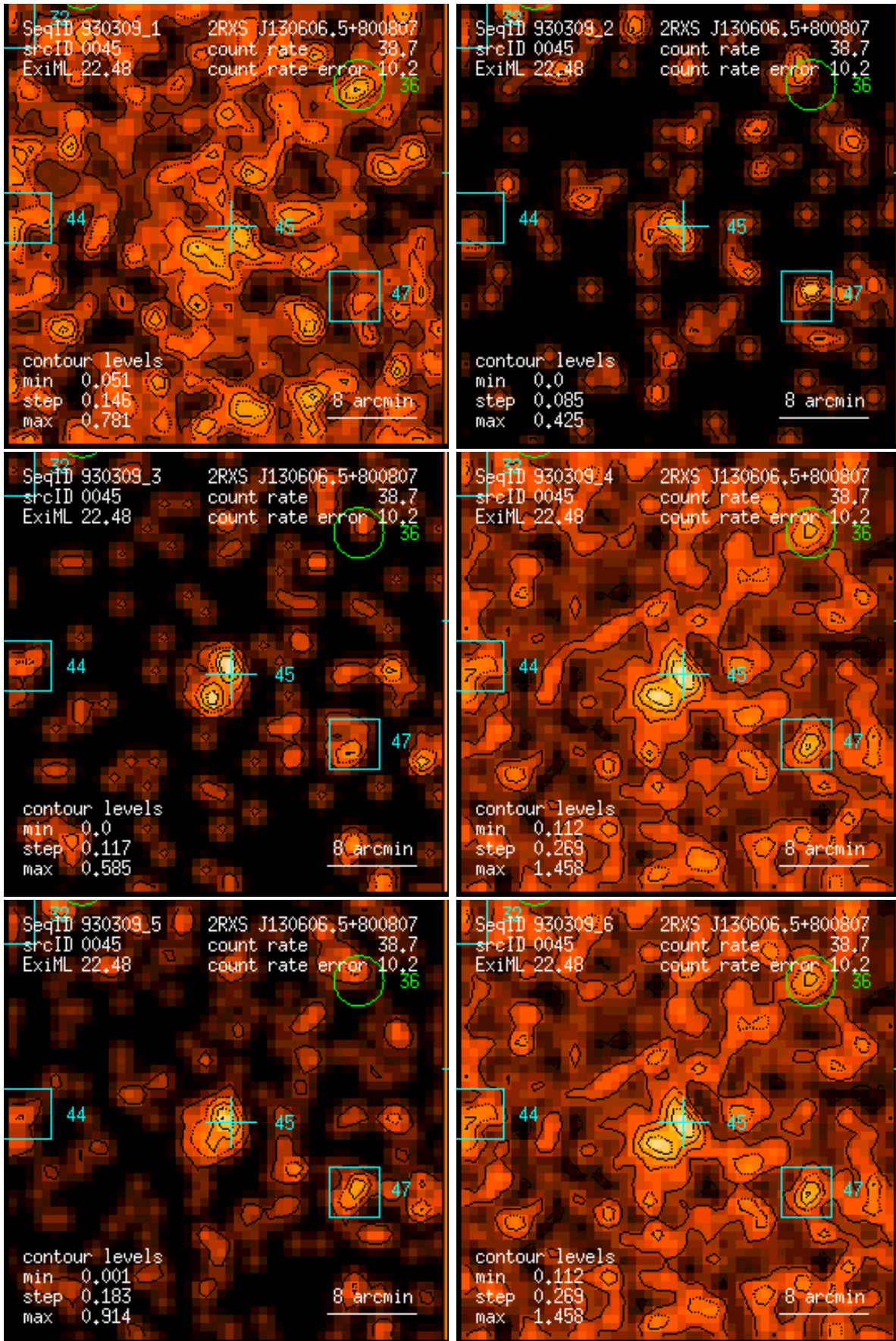
Figure 45: RASS 930309: detection 0045: band rate images, Gaussian filter: (1) PSPC channels 11 – 41, (2) 52 – 90, (3) 91 – 201, (4) 11 – 235, (5) 52 – 201, (6) 11 – 201. Broad band rates in counts/ks. Band rate contour levels in counts/ks/arcmin 2 .
