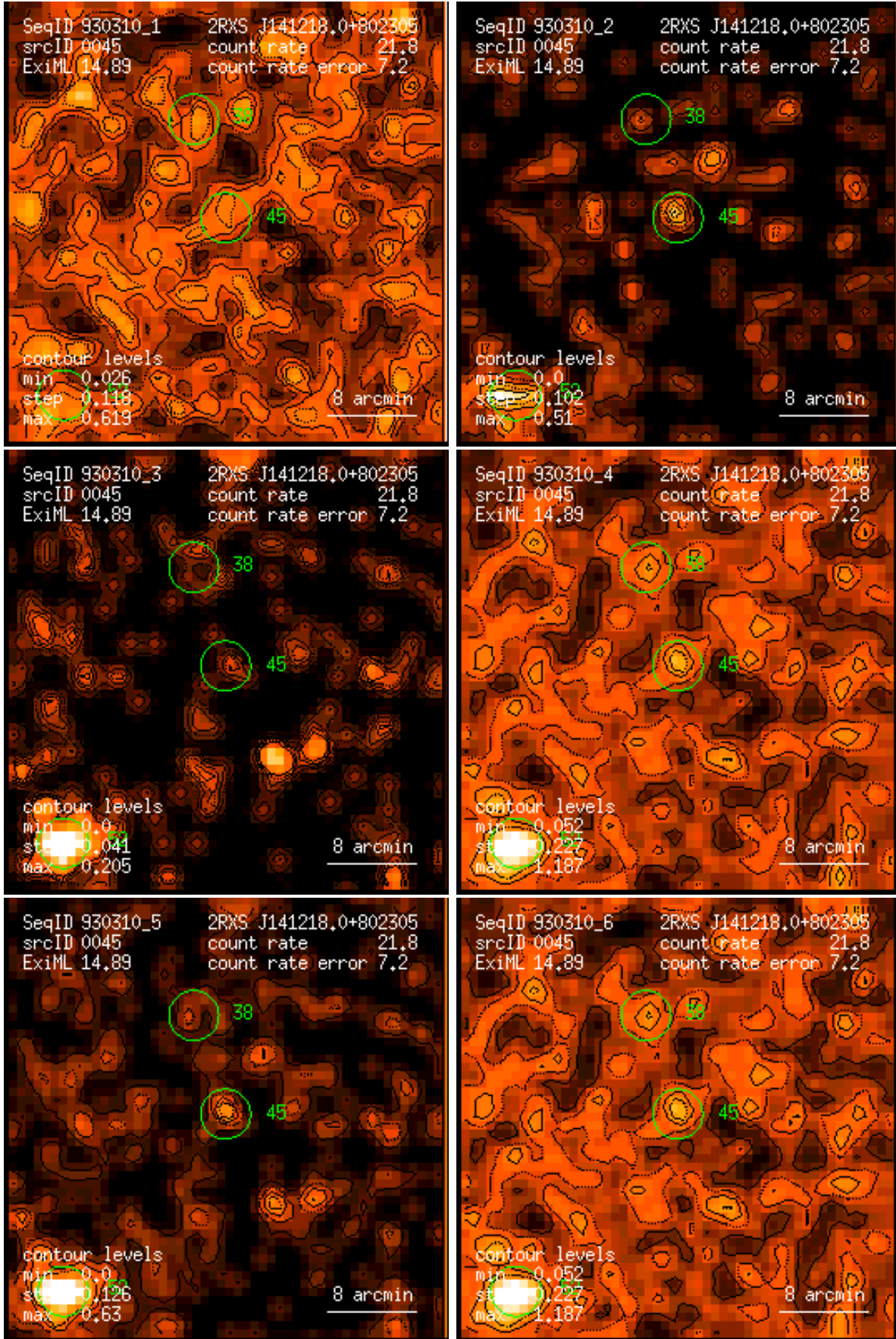
Figure 45: RASS 930310: detection 0045: band rate images, Gaussian filter: (1) PSPC channels 11 – 41, (2) 52 – 90, (3) 91 – 201, (4) 11 – 235, (5) 52 – 201, (6) 11 – 201. Broad band rates in counts/ks. Band rate contour levels in counts/ks/arcmin 2 .
