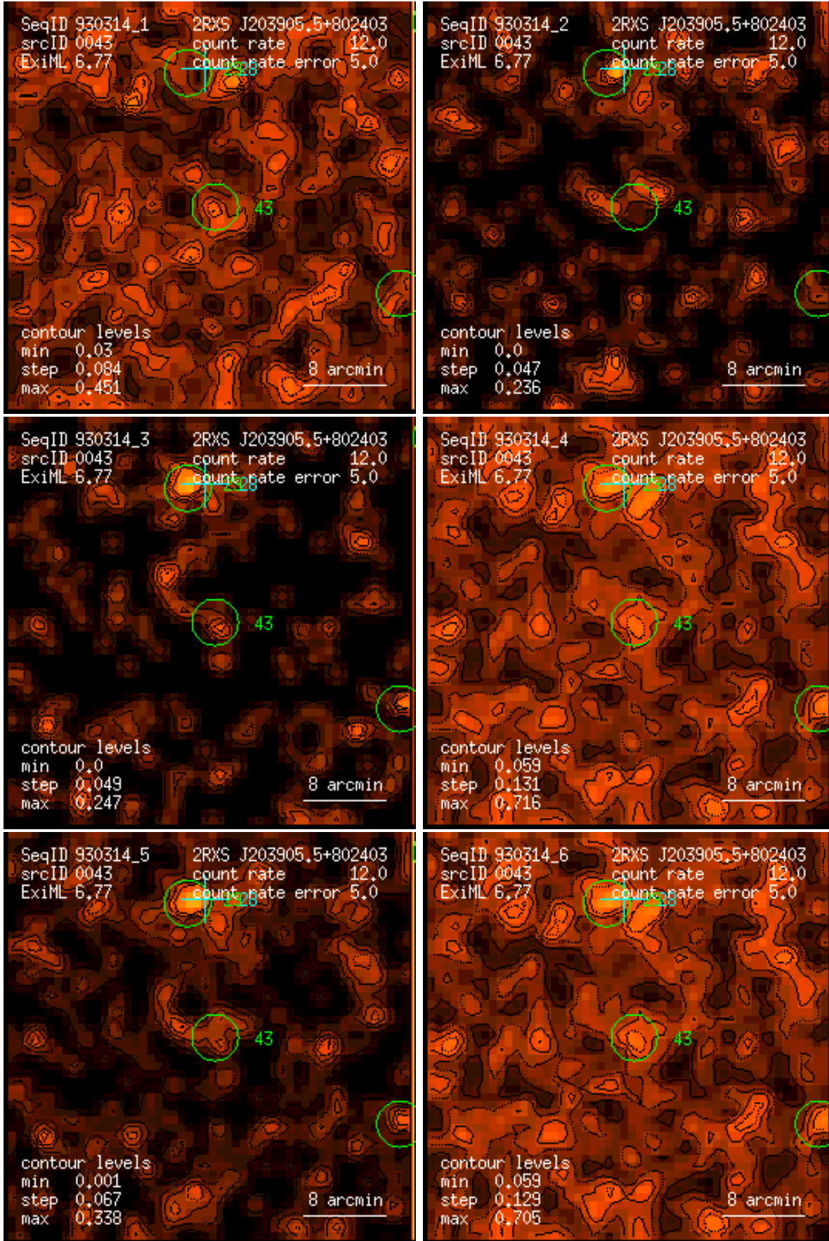
Figure 43: RASS 930314: detection 0043: band rate images, Gaussian filter: (1) PSPC channels 11 – 41, (2) 52 – 90, (3) 91 – 201, (4) 11 – 235, (5) 52 – 201, (6) 11 – 201. Broad band rates in counts/ks. Band rate contour levels in counts/ks/arcmin 2 .
