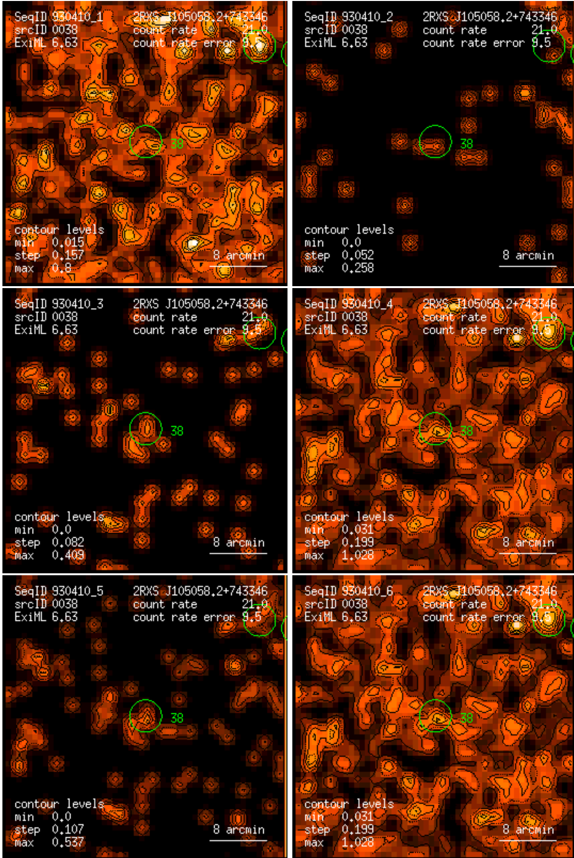
Figure 38: RASS 930410: detection 0038: band rate images, Gaussian filter: (1) PSPC channels 11 – 41, (2) 52 – 90, (3) 91 – 201, (4) 11 – 235, (5) 52 – 201, (6) 11 – 201. Broad band rates in counts/ks. Band rate contour levels in counts/ks/arcmin 2 .
