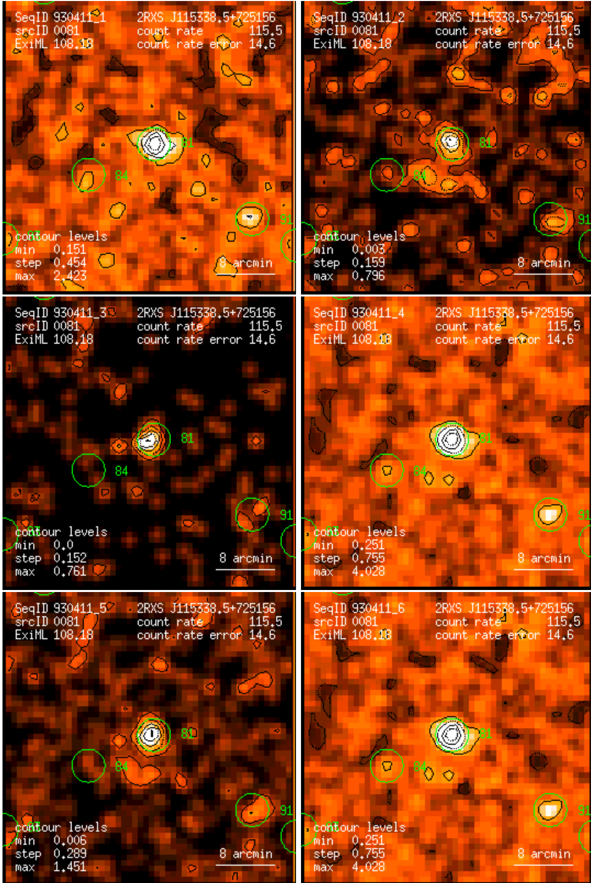
Figure 81: RASS 930411: detection 0081: band rate images, Gaussian filter: (1) PSPC channels 11 – 41, (2) 52 – 90, (3) 91 – 201, (4) 11 – 235, (5) 52 – 201, (6) 11 – 201. Broad band rates in counts/ks. Band rate contour levels in counts/ks/arcmin 2 .
