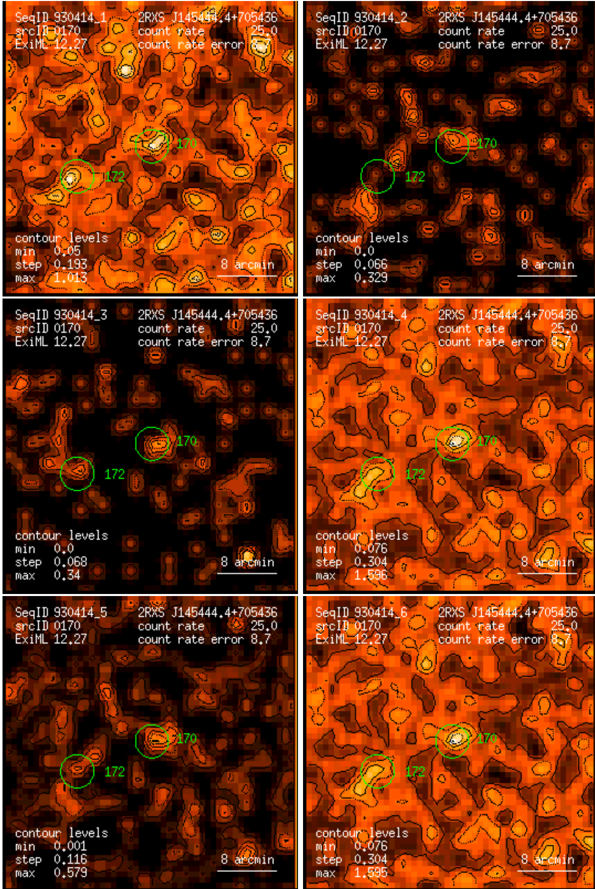
Figure 170: RASS 930414: detection 0170: band rate images, Gaussian filter: (1) PSPC channels 11 – 41, (2) 52 – 90, (3) 91 – 201, (4) 11 – 235, (5) 52 – 201, (6) 11 – 201. Broad band rates in counts/ks. Band rate contour levels in counts/ks/arcmin 2 .
