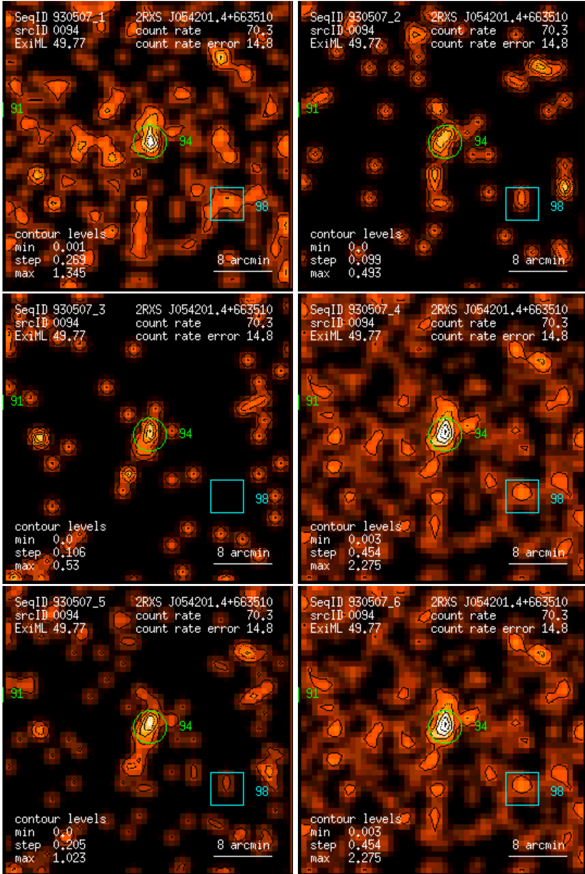
Figure 94: RASS 930507: detection 0094: band rate images, Gaussian filter: (1) PSPC channels 11 – 41, (2) 52 – 90, (3) 91 – 201, (4) 11 – 235, (5) 52 – 201, (6) 11 – 201. Broad band rates in counts/ks. Band rate contour levels in counts/ks/arcmin 2 .
