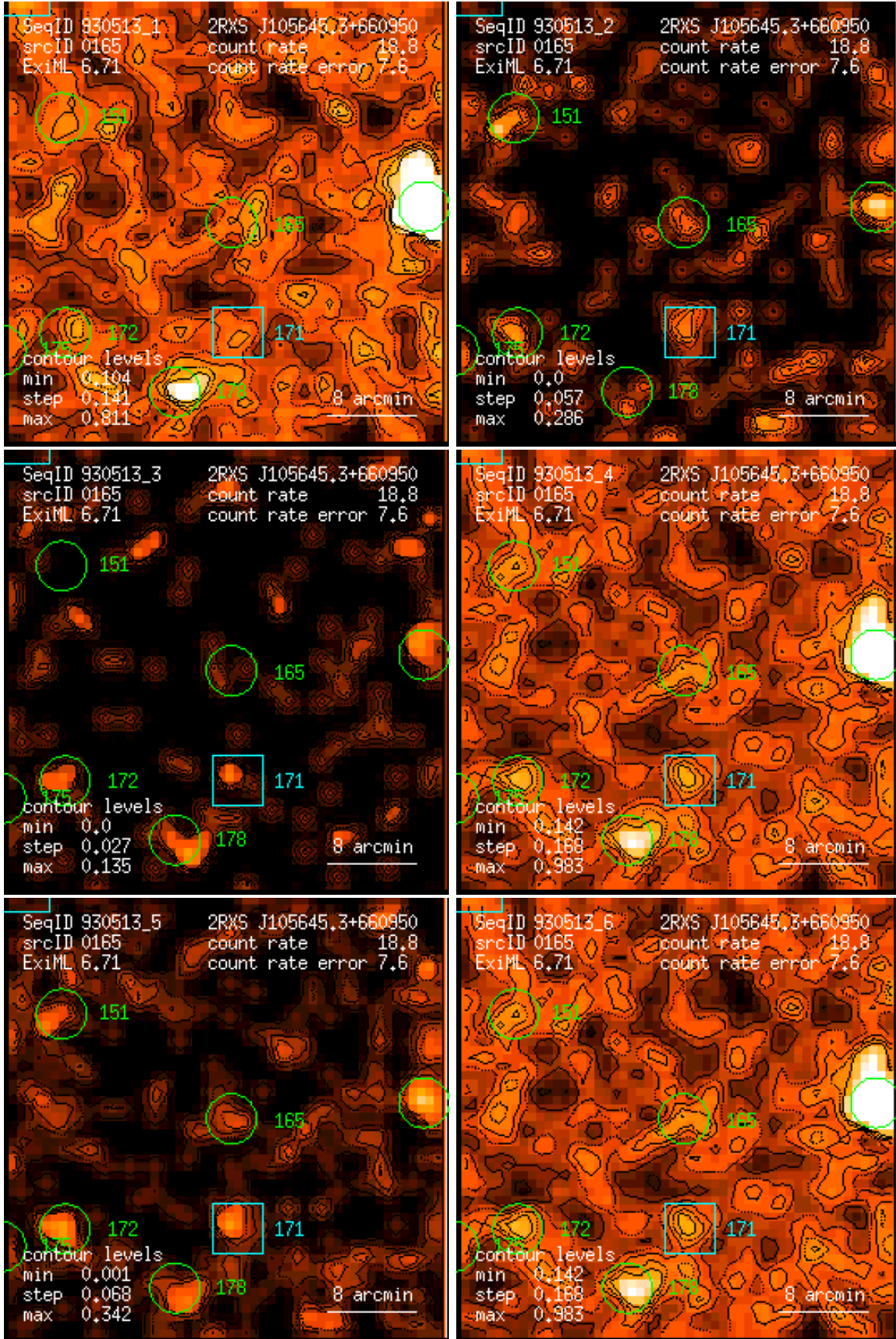
Figure 165: RASS 930513: detection 0165: band rate images, Gaussian filter: (1) PSPC channels 11 – 41, (2) 52 – 90, (3) 91 – 201, (4) 11 – 235, (5) 52 – 201, (6) 11 – 201. Broad band rates in counts/ks. Band rate contour levels in counts/ks/arcmin 2 .
