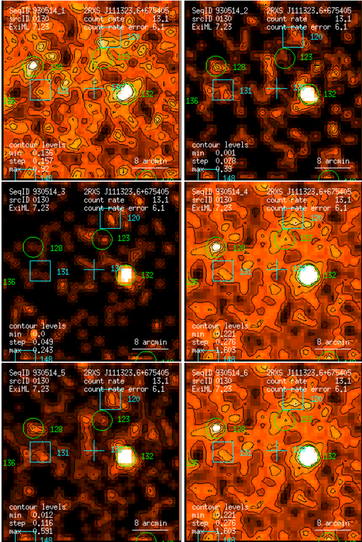
Figure 130: RASS 930514: detection 0130: band rate images, Gaussian filter: (1) PSPC channels 11 – 41, (2) 52 – 90, (3) 91 – 201, (4) 11 – 235, (5) 52 – 201, (6) 11 – 201. Broad band rates in counts/ks. Band rate contour levels in counts/ks/arcmin 2 .
