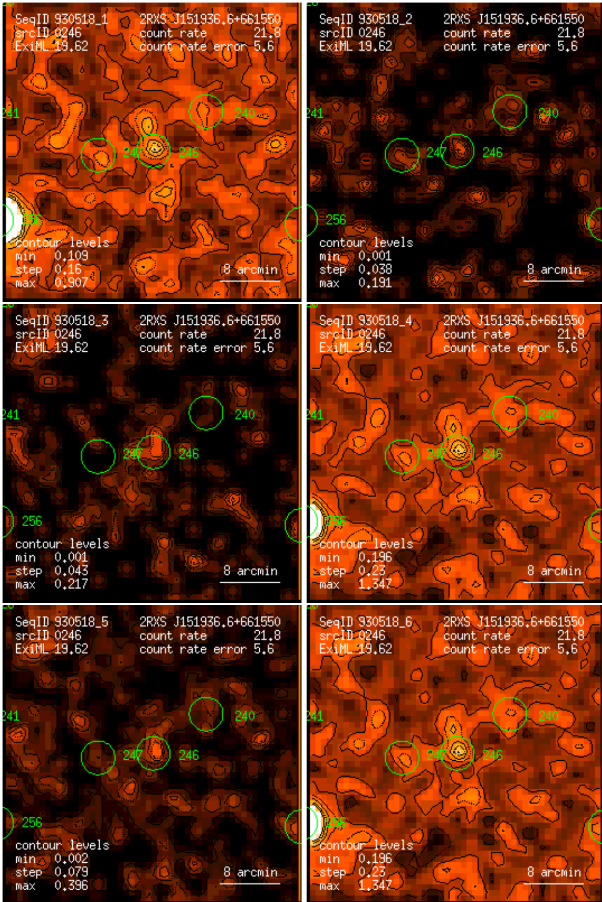
Figure 246: RASS 930518: detection 0246: band rate images, Gaussian filter: (1) PSPC channels 11 – 41, (2) 52 – 90, (3) 91 – 201, (4) 11 – 235, (5) 52 – 201, (6) 11 – 201. Broad band rates in counts/ks. Band rate contour levels in counts/ks/arcmin 2 .
