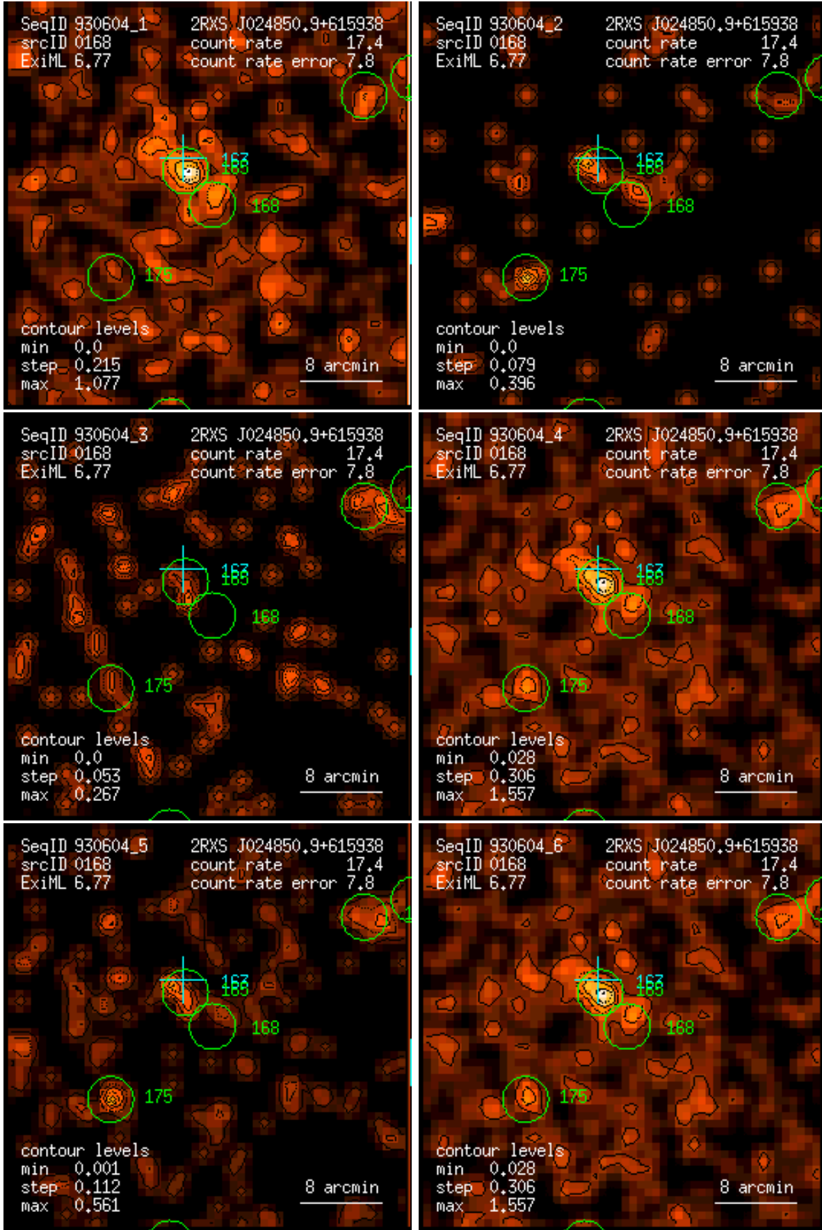
Figure 168: RASS 930604: detection 0168: band rate images, Gaussian filter: (1) PSPC channels 11 – 41, (2) 52 – 90, (3) 91 – 201, (4) 11 – 235, (5) 52 – 201, (6) 11 – 201. Broad band rates in counts/ks. Band rate contour levels in counts/ks/arcmin 2 .
