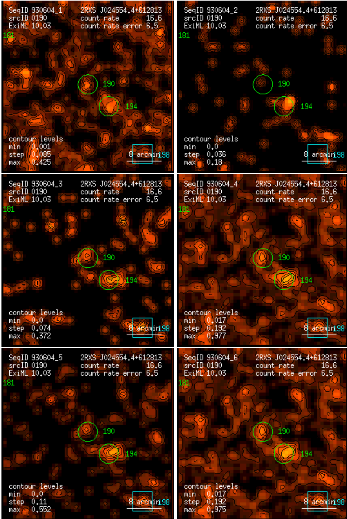
Figure 190: RASS 930604: detection 0190: band rate images, Gaussian filter: (1) PSPC channels 11 – 41, (2) 52 – 90, (3) 91 – 201, (4) 11 – 235, (5) 52 – 201, (6) 11 – 201. Broad band rates in counts/ks. Band rate contour levels in counts/ks/arcmin 2 .
