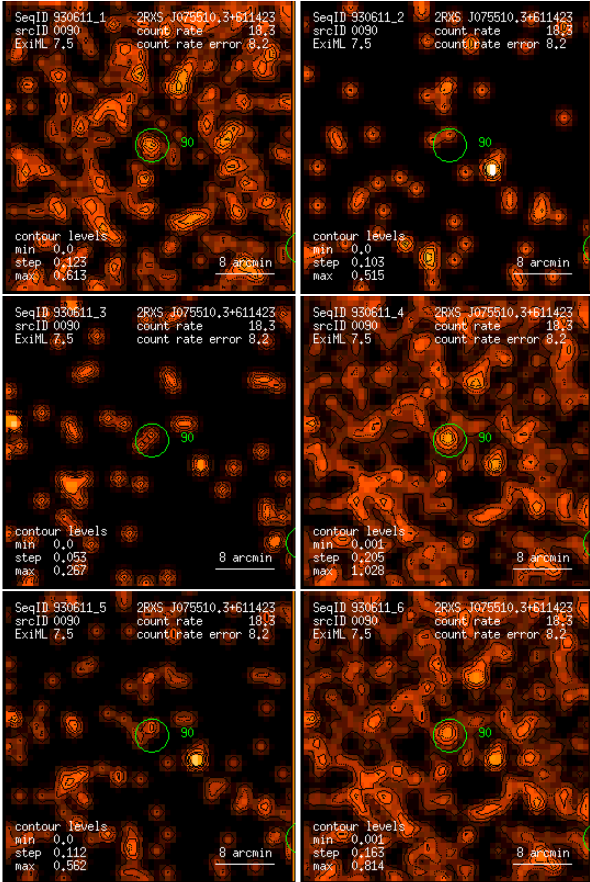
Figure 90: RASS 930611: detection 0090: band rate images, Gaussian filter: (1) PSPC channels 11 – 41, (2) 52 – 90, (3) 91 – 201, (4) 11 – 235, (5) 52 – 201, (6) 11 – 201. Broad band rates in counts/ks. Band rate contour levels in counts/ks/arcmin 2 .
