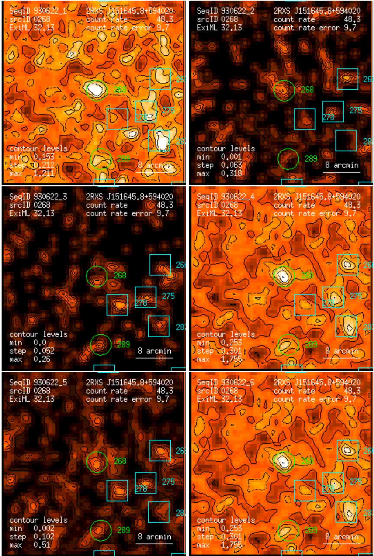
Figure 268: RASS 930622: detection 0268: band rate images, Gaussian filter: (1) PSPC channels 11 – 41, (2) 52 – 90, (3) 91 – 201, (4) 11 – 235, (5) 52 – 201, (6) 11 – 201. Broad band rates in counts/ks. Band rate contour levels in counts/ks/arcmin 2 .
