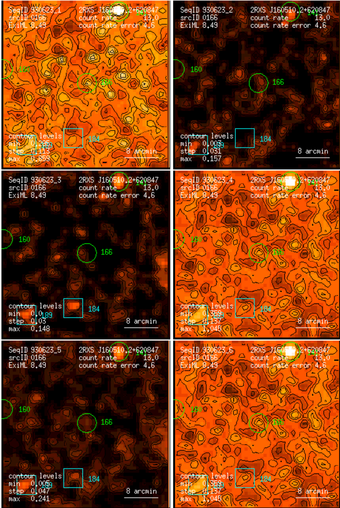
Figure 166: RASS 930623: detection 0166: band rate images, Gaussian filter: (1) PSPC channels 11 – 41, (2) 52 – 90, (3) 91 – 201, (4) 11 – 235, (5) 52 – 201, (6) 11 – 201. Broad band rates in counts/ks. Band rate contour levels in counts/ks/arcmin 2 .
