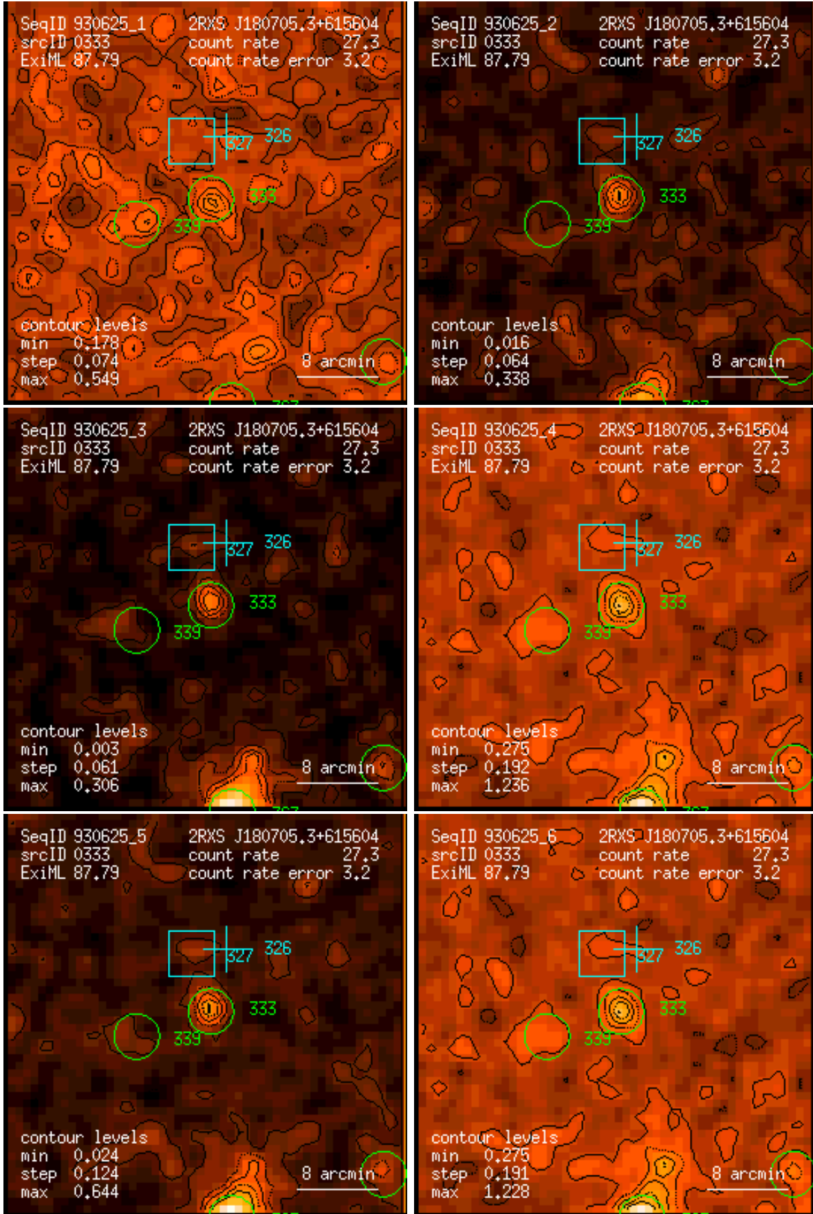
Figure 333: RASS 930625: detection 0333: band rate images, Gaussian filter: (1) PSPC channels 11 – 41, (2) 52 – 90, (3) 91 – 201, (4) 11 – 235, (5) 52 – 201, (6) 11 – 201. Broad band rates in counts/ks. Band rate contour levels in counts/ks/arcmin 2 .
