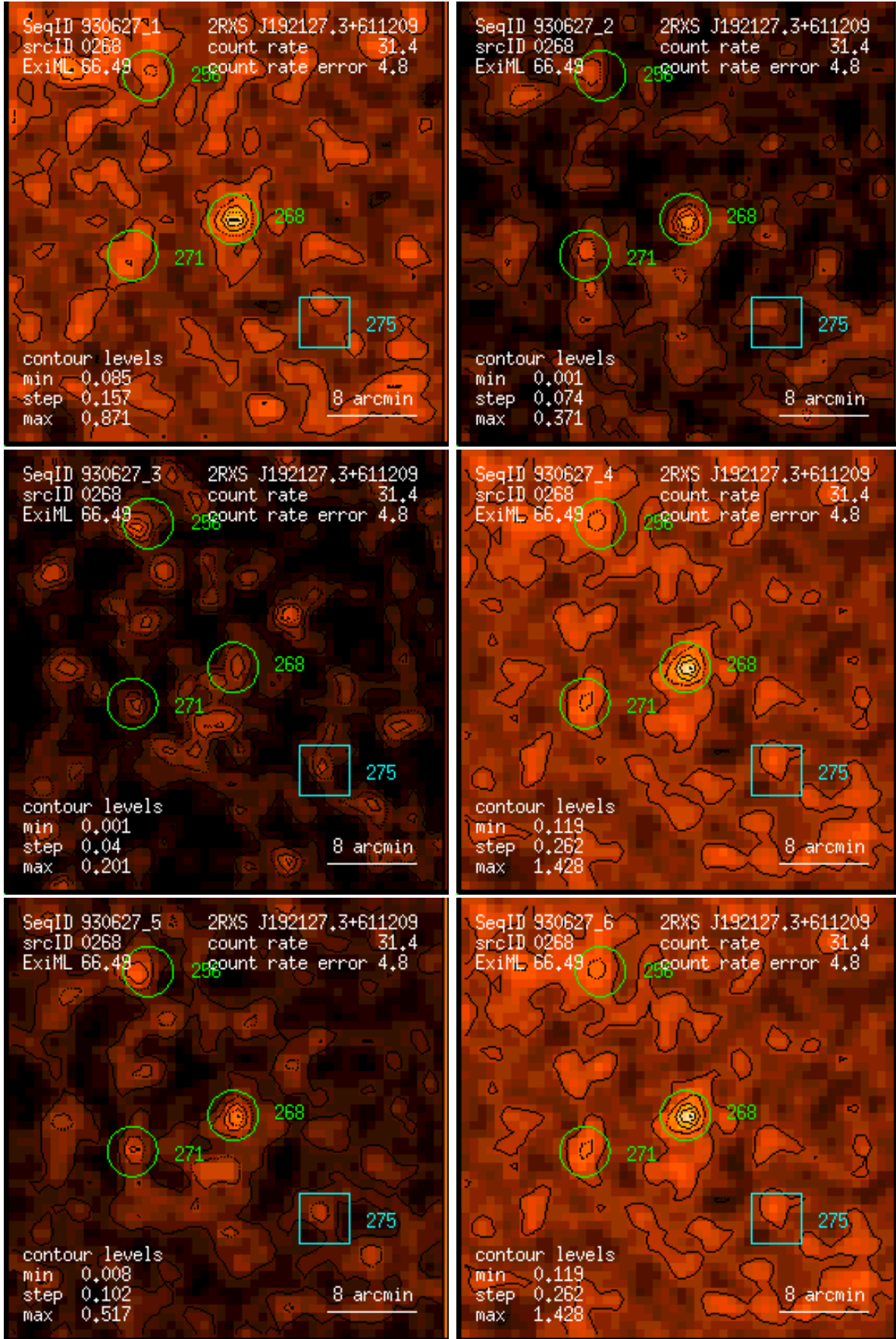
Figure 268: RASS 930627: detection 0268: band rate images, Gaussian filter: (1) PSPC channels 11 – 41, (2) 52 – 90, (3) 91 – 201, (4) 11 – 235, (5) 52 – 201, (6) 11 – 201. Broad band rates in counts/ks. Band rate contour levels in counts/ks/arcmin 2 .
