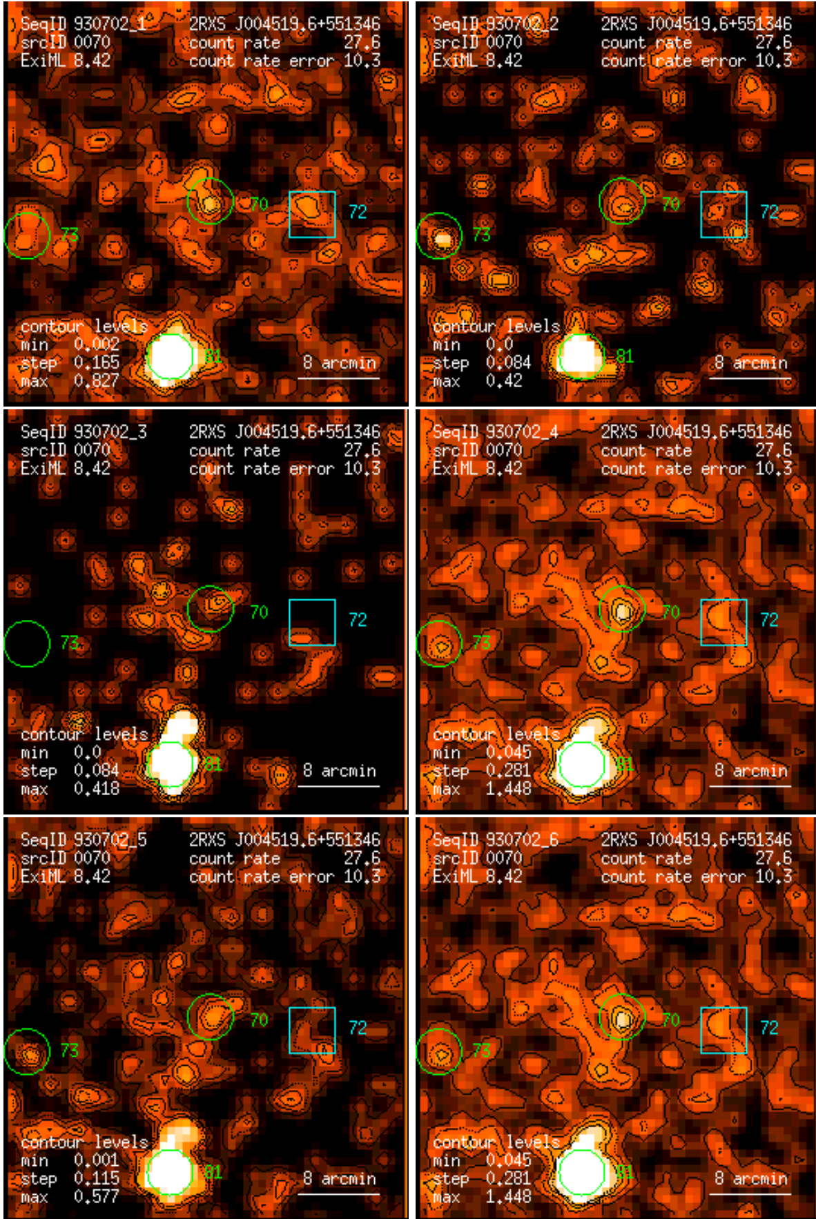
Figure 70: RASS 930702: detection 0070: band rate images, Gaussian filter: (1) PSPC channels 11 – 41, (2) 52 – 90, (3) 91 – 201, (4) 11 – 235, (5) 52 – 201, (6) 11 – 201. Broad band rates in counts/ks. Band rate contour levels in counts/ks/arcmin 2 .
