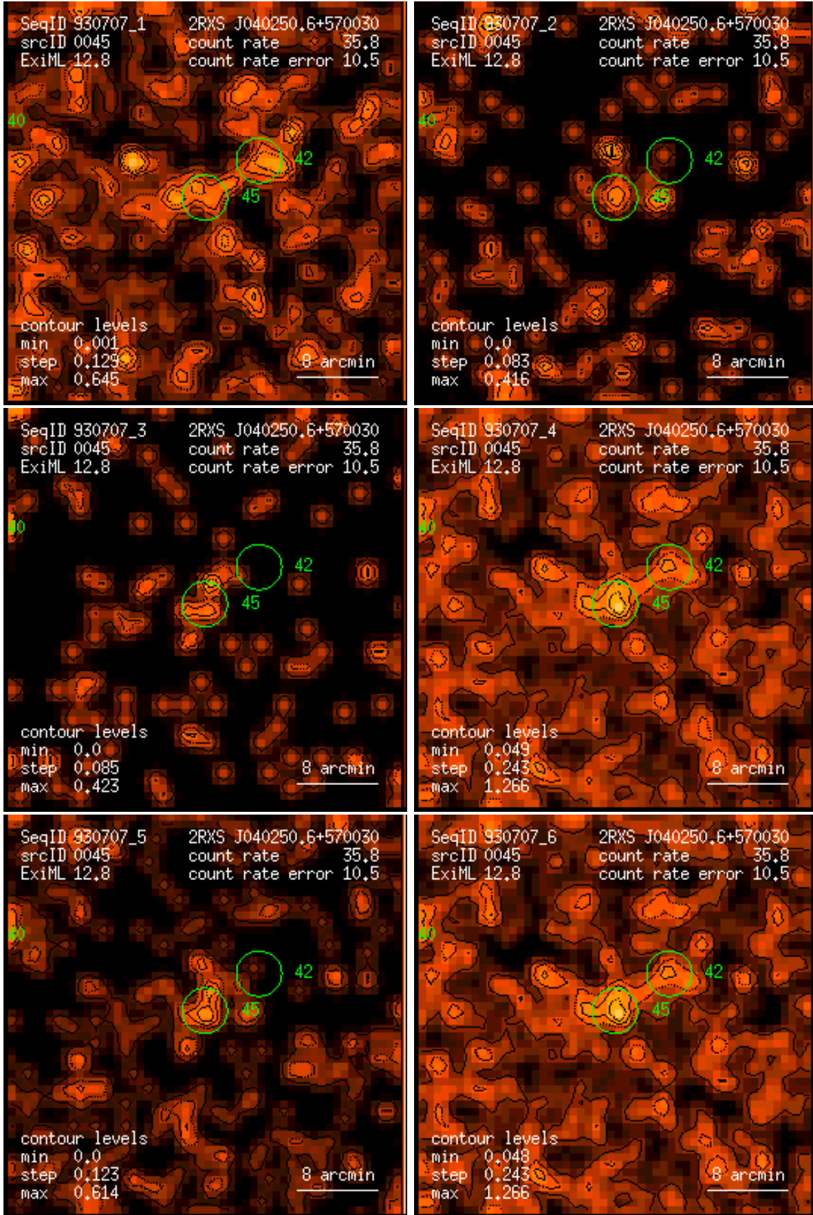
Figure 45: RASS 930707: detection 0045: band rate images, Gaussian filter: (1) PSPC channels 11 – 41, (2) 52 – 90, (3) 91 – 201, (4) 11 – 235, (5) 52 – 201, (6) 11 – 201. Broad band rates in counts/ks. Band rate contour levels in counts/ks/arcmin 2 .
