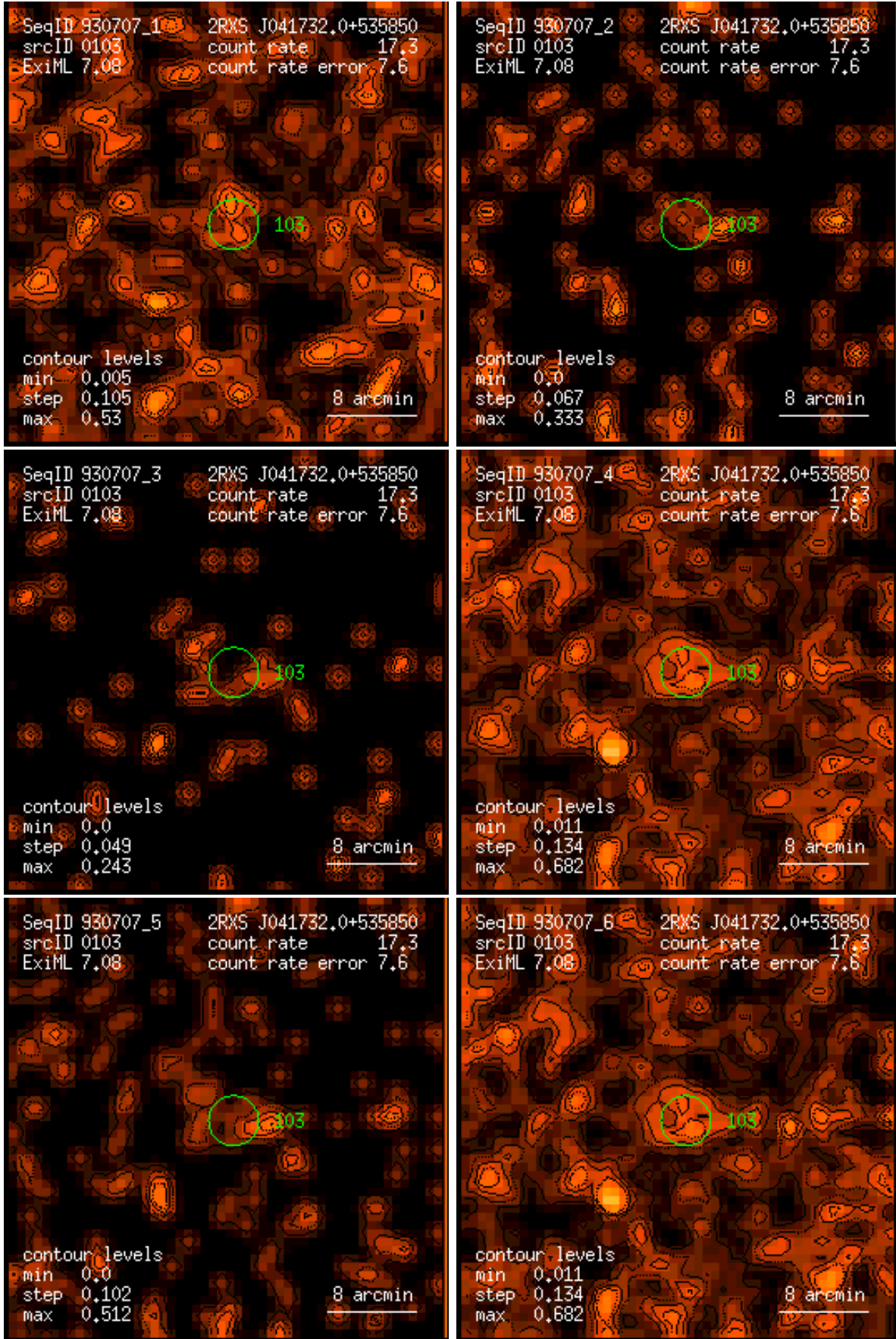
Figure 103: RASS 930707: detection 0103: band rate images, Gaussian filter: (1) PSPC channels 11 – 41, (2) 52 – 90, (3) 91 – 201, (4) 11 – 235, (5) 52 – 201, (6) 11 – 201. Broad band rates in counts/ks. Band rate contour levels in counts/ks/arcmin 2 .
