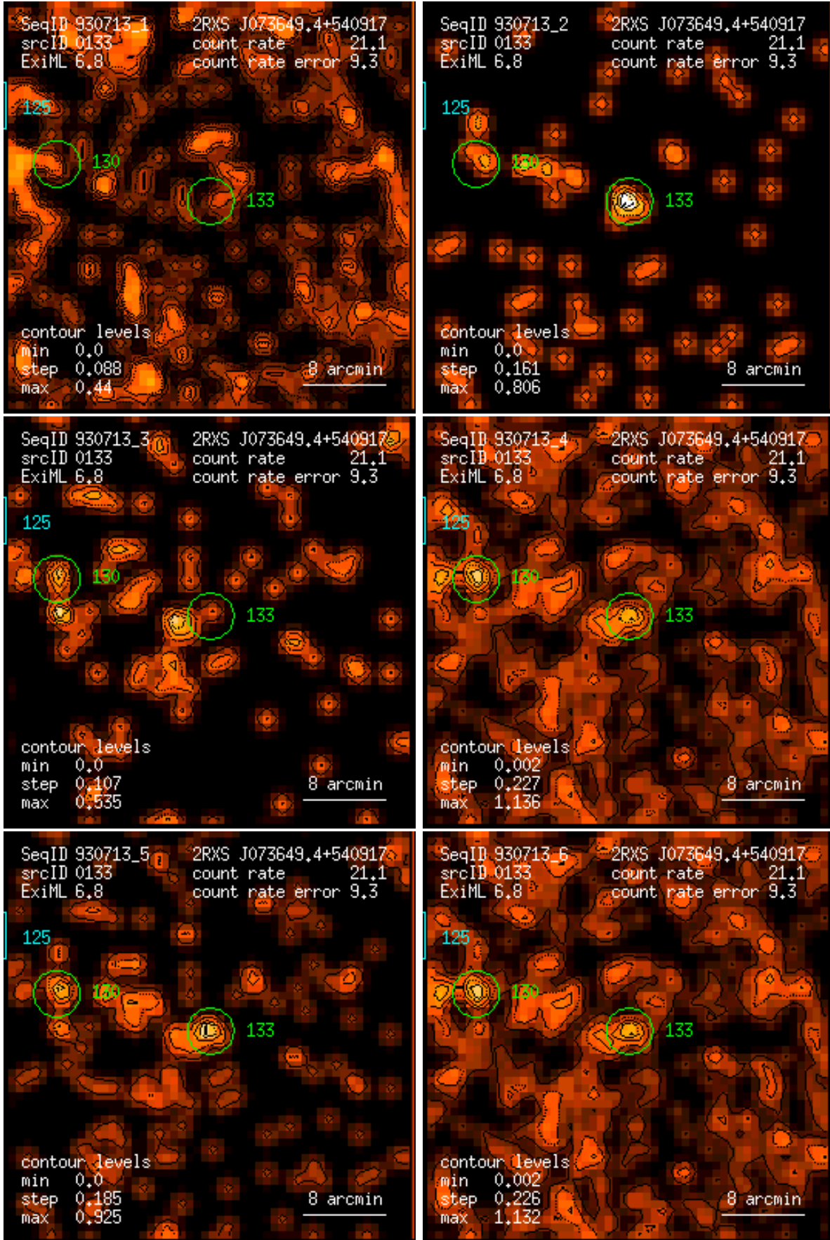
Figure 133: RASS 930713: detection 0133: band rate images, Gaussian filter: (1) PSPC channels 11 – 41, (2) 52 – 90, (3) 91 – 201, (4) 11 – 235, (5) 52 – 201, (6) 11 – 201. Broad band rates in counts/ks. Band rate contour levels in counts/ks/arcmin 2 .
