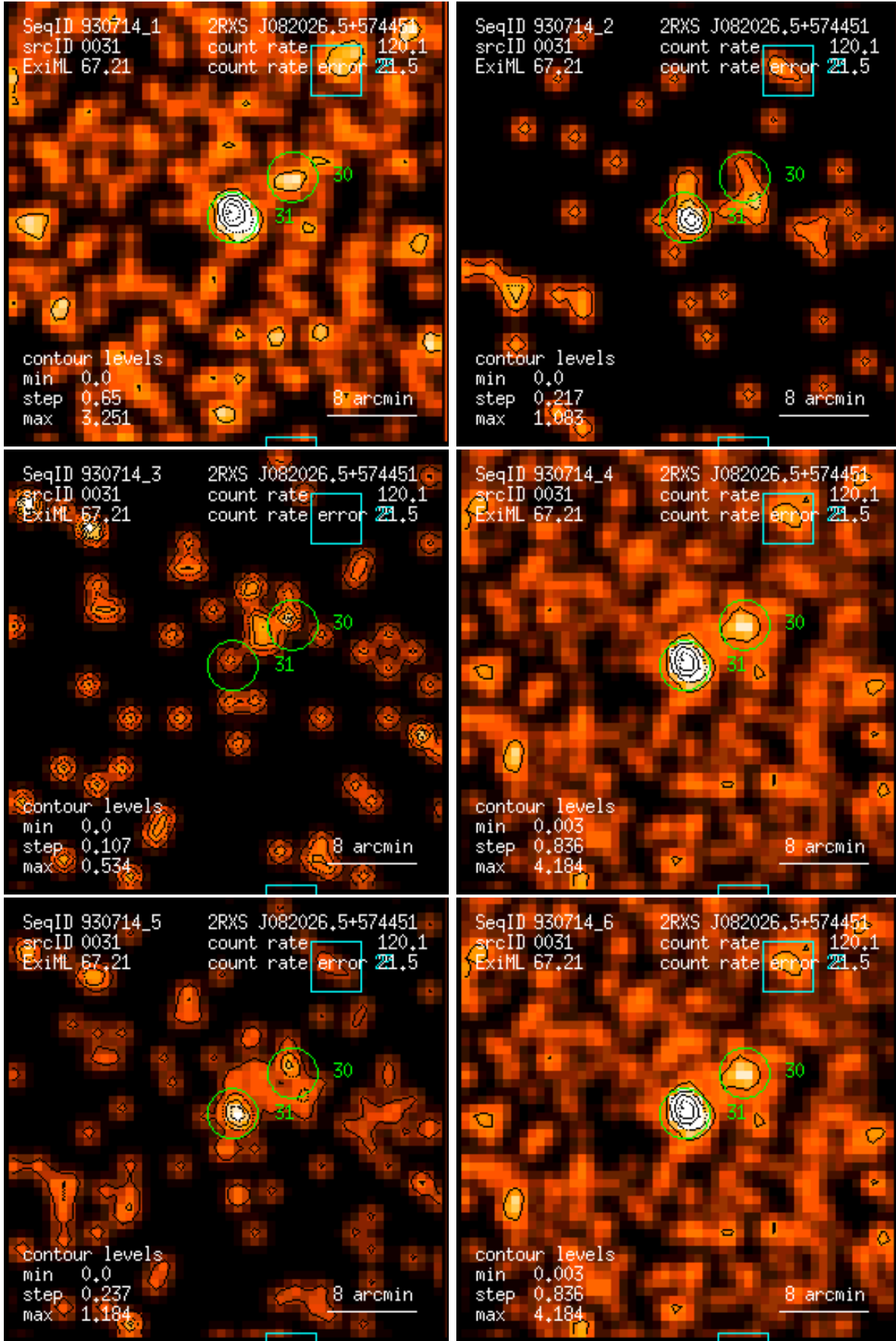
Figure 31: RASS 930714: detection 0031: band rate images, Gaussian filter: (1) PSPC channels 11 – 41, (2) 52 – 90, (3) 91 – 201, (4) 11 – 235, (5) 52 – 201, (6) 11 – 201. Broad band rates in counts/ks. Band rate contour levels in counts/ks/arcmin 2 .
